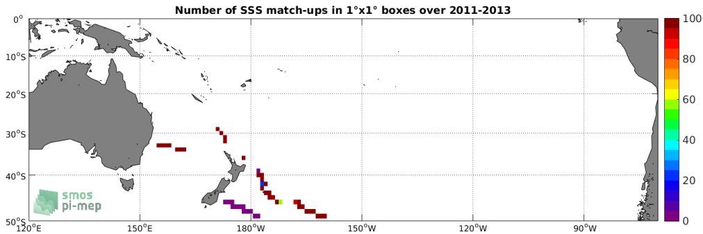
Figure 4: Number of SSS match-ups between TSG-GOSUD-Sailing-ship SSS and the Aquarius-L3-JPL-V5-7DAY-RUNNING SSS product for the South Pacific Ocean Pi-MEP region over 1^\circ \times 1^\circ boxes and for the full satellite product period.
