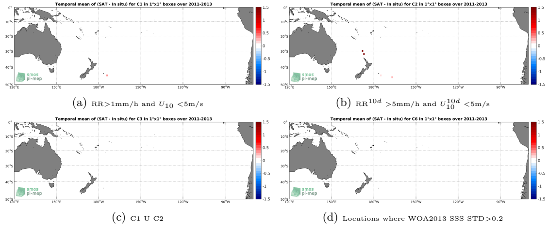
Figure 12: Temporal mean gridded over spatial boxes of size 1^\circ \times 1^\circ of \Delta SSS (Aquarius-L3-JPL-V5-7DAY-RUNNING - TSG-GOSUD-Sailing-ship) for 4 different subdatasets corresponding to:RR > 1 mm/h and U_{10} < 5 m/s (a), RR^{10d} > 5 mm/h and U_{10}^{10d} < 5 m/s (b), C1 U C2 (c),Locations where WOA2013 SSS STD > 0.2 (d).
