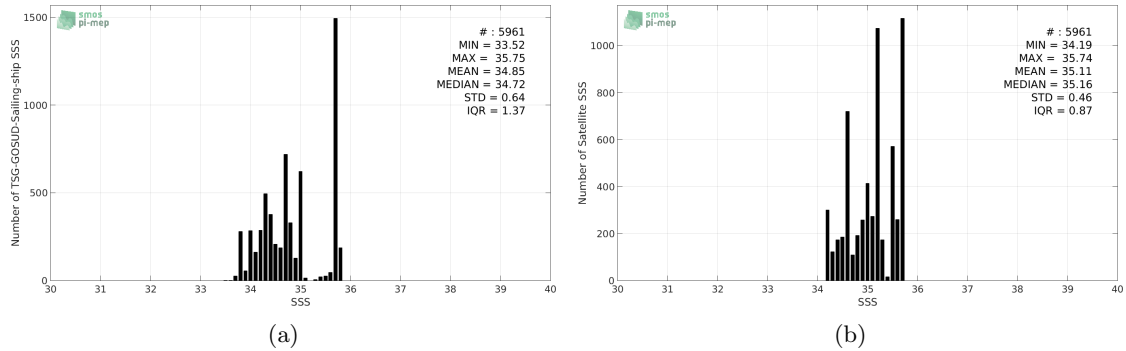
Figure 2: Histograms of SSS from TSG-GOSUD-Sailing-ship (a) and Aquarius-L3-JPL-V5-7DAY-RUNNING (b) considering all match-up pairs per bins of 0.1 over the South Pacific Ocean Pi-MEP region and for the full satellite product period.
