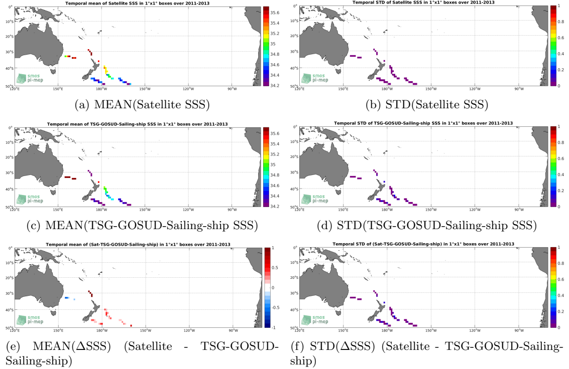
Figure 6: Temporal mean (left) and STD (right) of SSS from Aquarius-L3-JPL-V5-7DAY-RUNNING (top), TSG-GOSUD-Sailing-ship (middle), and of \Delta SSS (Satellite - TSG-GOSUD-Sailing-ship). Only match-up pairs are used to generate these maps.
