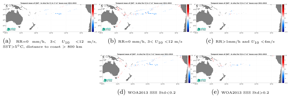
Figure 14: Temporal mean gridded over spatial boxes of size 1^\circ \times 1^\circ of \Delta SSS (Aquarius SSS L3 CAP v5 - 7-Day running (JPL) - TSG (GOSUD-Research-vessel)) for 5 different subdatasets corresponding to:RR=0 mm/h, 3 < U_{10} < 12 m/s, SST >5^\circ\text{C} , distance to coast > 800 km (a), RR=0 mm/h, 3 < U_{10} < 12 m/s (b), RR >1 mm/h and U_{10} < 4 m/s (c), WOA2013 SSS Std <0.2 (d), WOA2013 SSS Std >0.2 (e).
