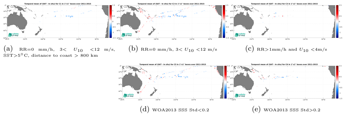
Figure 14: Temporal mean gridded over spatial boxes of size 1^\circ \times 1^\circ of \Delta\text{SSS} (Aquarius SSS L3 CAP v5 - 7-Day running (JPL) - TSG (GOSUD-Research-vessel)) for 5 different subdatasets corresponding to:RR=0 mm/h, 3 < U_{10} < 12 m/s, SST >5^\circ\text{C} , distance to coast > 800 km (a), RR=0 mm/h, 3 < U_{10} < 12 m/s (b), RR >1 mm/h and U_{10} < 4 m/s (c), WOA2013 SSS Std <0.2 (d), WOA2013 SSS Std >0.2 (e).
