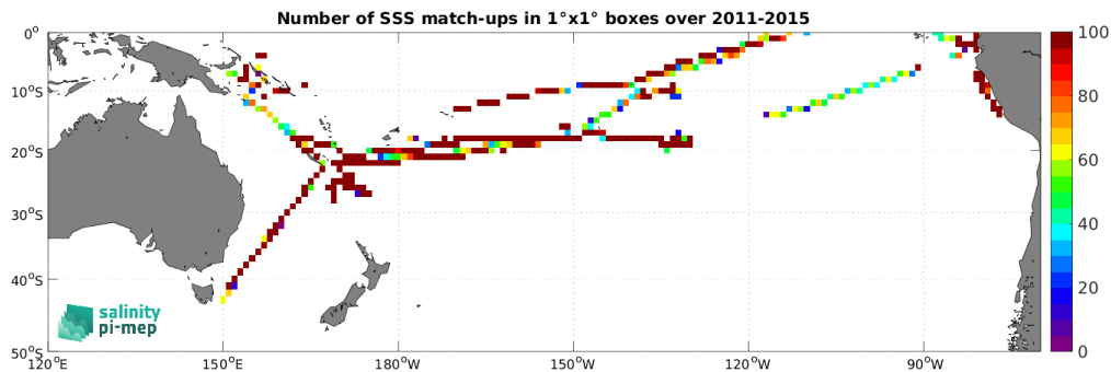
Figure 5: Number of SSS match-ups between TSG (GOSUD-Research-vessel) SSS and the Aquarius SSS L3 CAP v5 - 7-Day running (JPL) SSS product for the South Pacific Ocean Pi-MEP region over 1^\circ \times 1^\circ boxes and for the full satellite product period.
