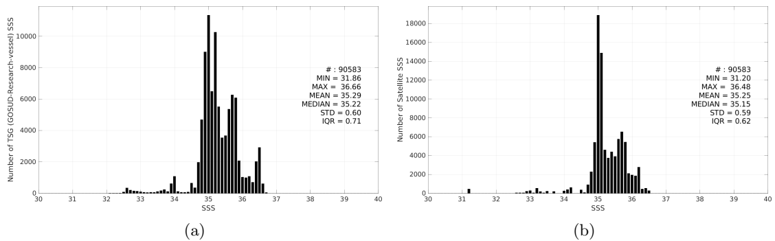
Figure 3: Histograms of SSS from TSG (GOSUD-Research-vessel) (a) and Aquarius SSS L3 CAP v5 - 7-Day running (JPL) (b) considering all match-up pairs per bins of 0.1 over the South Pacific Ocean Pi-MEP region and for the full satellite product period.
