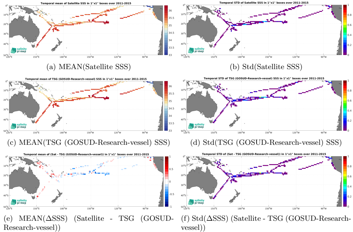
Figure 7: Temporal mean (left) and Std (right) of SSS from Aquarius SSS L3 CAP v5 - 7-Day running (JPL) (top), TSG (GOSUD-Research-vessel) (middle), and of \Delta SSS (Satellite - TSG (GOSUD-Research-vessel)). Only match-up pairs are used to generate these maps.
