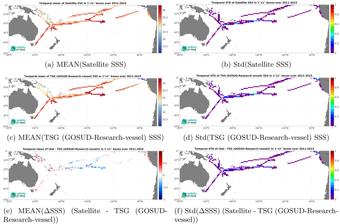
Figure 6: Temporal mean (left) and Std (right) of SSS from Aquarius SSS L3 CAP v5 - 7-Day running (JPL) (top), TSG (GOSUD-Research-vessel) (middle), and of \Delta SSS (Satellite - TSG (GOSUD-Research-vessel)). Only match-up pairs are used to generate these maps.
