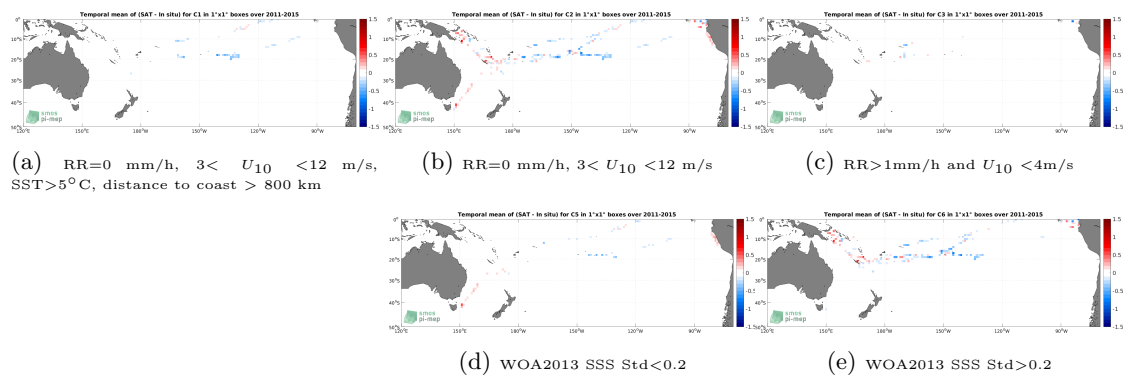
Figure 12: Temporal mean gridded over spatial boxes of size 1^\circ \times 1^\circ of \Delta SSS (Aquarius SSS L3 CAP v5 - 7-Day running (JPL) - TSG (GOSUD-Research-vessel)) for 5 different subdatasets corresponding to:RR=0 mm/h, 3 < U_{10} < 12 m/s, SST >5^\circ\text{C} , distance to coast > 800 km (a), RR=0 mm/h, 3 < U_{10} < 12 m/s (b), RR >1 mm/h and U_{10} < 4 m/s (c), WOA2013 SSS Std <0.2 (d), WOA2013 SSS Std >0.2 (e).
