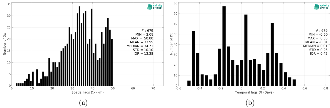
Figure 6: Histograms of the spatial (a) and temporal (b) lags between the location/time of the Marine mammals measurement and the date of the corresponding Aquarius SSS L3 CAP v5 - 7-Day running (JPL) SSS pixel.
