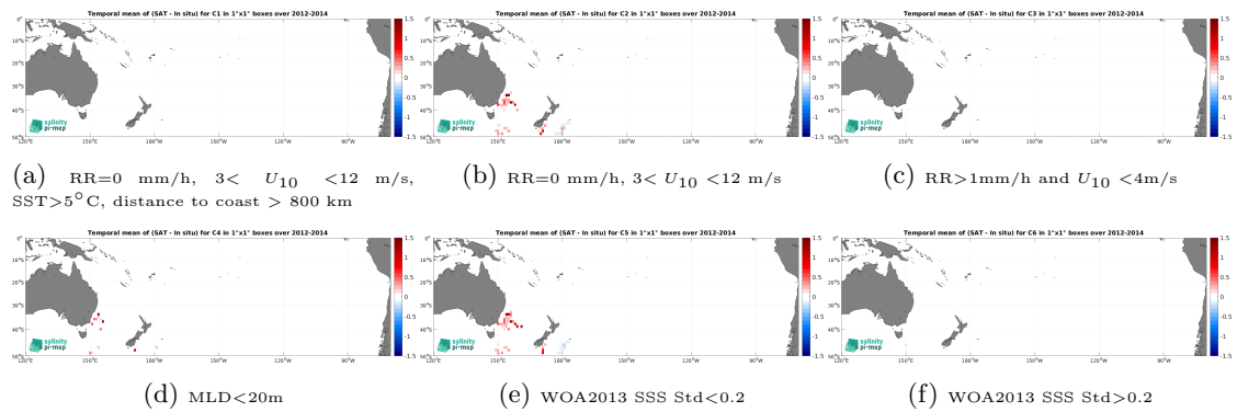
Figure 14: Temporal mean gridded over spatial boxes of size 1^\circ \times 1^\circ of \Delta SSS (Aquarius SSS L3 CAP v5 - 7-Day running (JPL) - Marine mammals) for 6 different subdatasets corresponding to:RR=0 mm/h, 3 < U_{10} < 12 m/s, SST >5^\circ C, distance to coast > 800 km (a), RR=0 mm/h, 3 < U_{10} < 12 m/s (b), RR >1 mm/h and U_{10} < 4 m/s (c),MLD <20 m (d),WOA2013 SSS Std <0.2 (e),WOA2013 SSS Std >0.2 (f).
