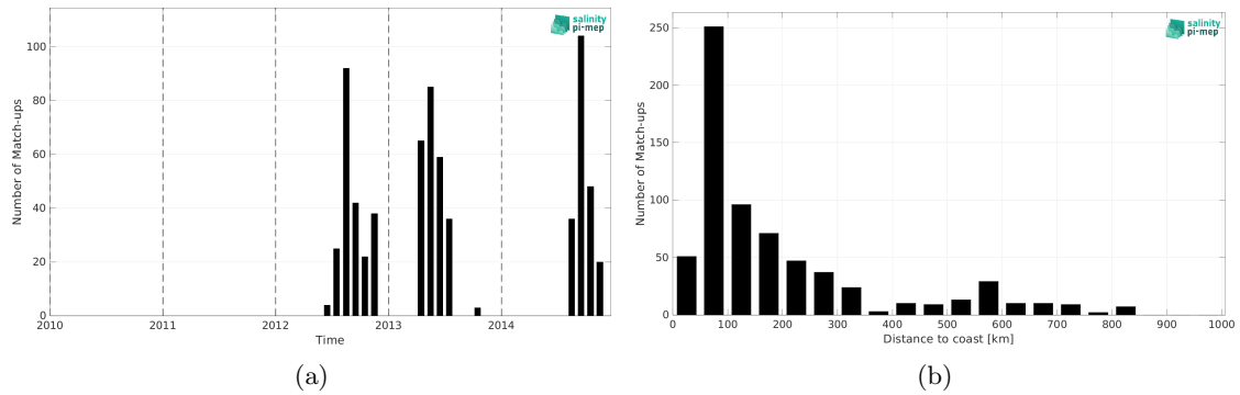
Figure 2: Number of match-ups between Marine mammals and Aquarius SSS L3 CAP v5 - 7-Day running (JPL) SSS as a function of time (a) and as function of the distance to coast (b) over the South Pacific Ocean Pi-MEP region and for the full satellite product period.
