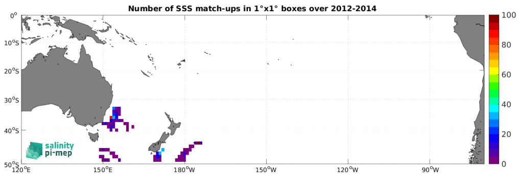
Figure 5: Number of SSS match-ups between Marine mammals SSS and the Aquarius SSS L3 CAP v5 - 7-Day running (JPL) SSS product for the South Pacific Ocean Pi-MEP region over 1^\circ \times 1^\circ boxes and for the full satellite product period.
