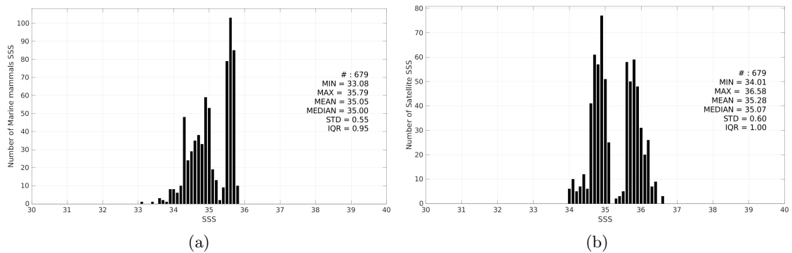
Figure 3: Histograms of SSS from Marine mammals (a) and Aquarius SSS L3 CAP v5 - 7-Day running (JPL) (b) considering all match-up pairs per bins of 0.1 over the South Pacific Ocean Pi-MEP region and for the full satellite product period.
