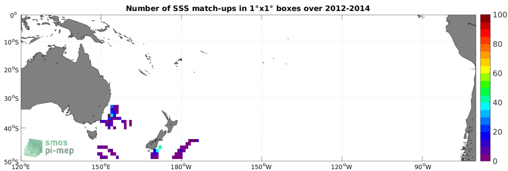
Figure 4: Number of SSS match-ups between Marine mammals SSS and the Aquarius SSS L3 CAP v5 - 7-Day running (JPL) SSS product for the South Pacific Ocean Pi-MEP region over 1^{\circ} \times 1^{\circ} boxes and for the full satellite product period.
