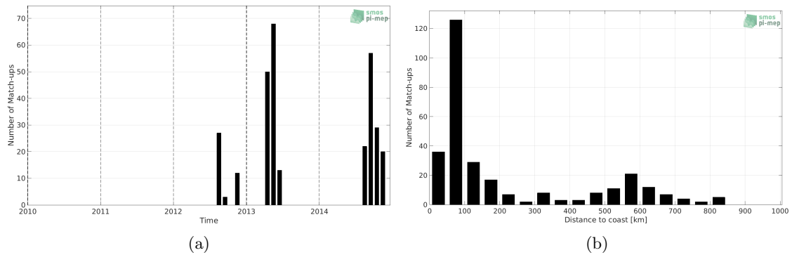
Figure 1: Number of match-ups between Sea mammals and Aquarius SSS L3 CAP v5 - 7-Day running (JPL) SSS as a function of time (a) and as function of the distance to coast (b) over the South Pacific Ocean Pi-MEP region and for the full satellite product period.
