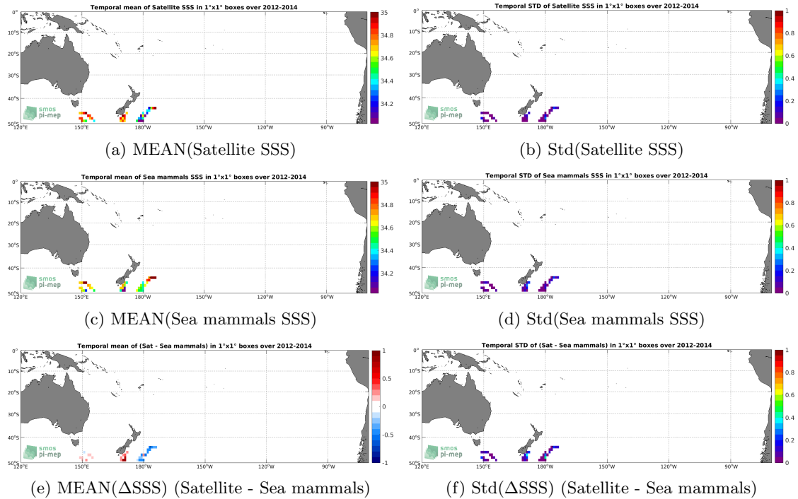
Figure 6: Temporal mean (left) and Std (right) of SSS from Aquarius SSS L3 CAP v5 - 7-Day running (JPL) (top), Sea mammals (middle), and of \Delta SSS (Satellite - Sea mammals). Only match-up pairs are used to generate these maps.
