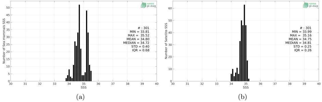
Figure 2: Histograms of SSS from Sea mammals (a) and Aquarius SSS L3 CAP v5 - 7-Day running (JPL) (b) considering all match-up pairs per bins of 0.1 over the South Pacific Ocean Pi-MEP region and for the full satellite product period.
