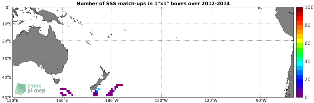
Figure 4: Number of SSS match-ups between Sea mammals SSS and the Aquarius SSS L3 CAP v5 - 7-Day running (JPL) SSS product for the South Pacific Ocean Pi-MEP region over 1^\circ \times 1^\circ boxes and for the full satellite product period.
