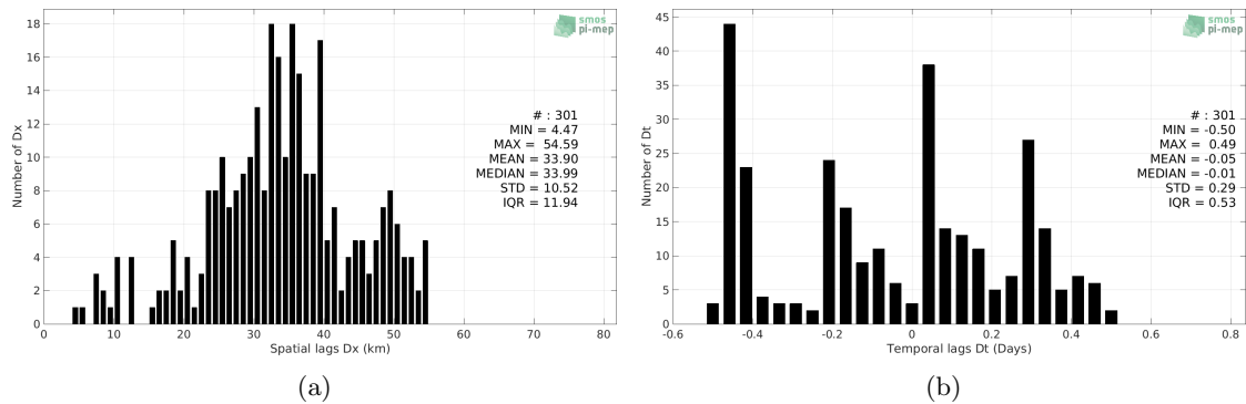
Figure 5: Histograms of the spatial (a) and temporal (b) lags between the time of the Sea mammals measurements and the date of the corresponding Aquarius SSS L3 CAP v5 - 7-Day running (JPL) SSS product.
