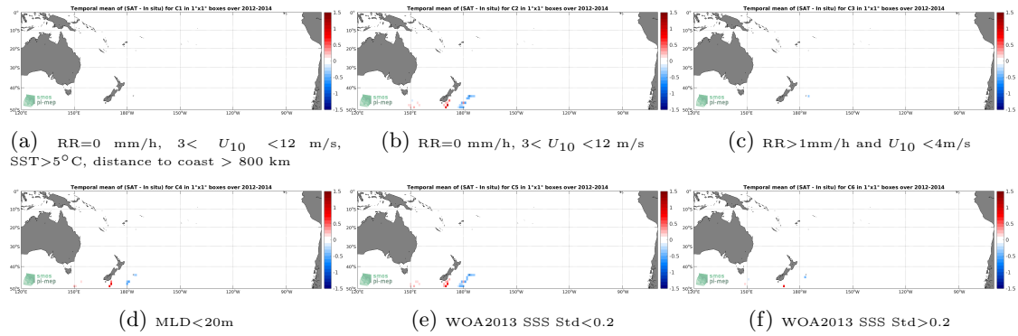
Figure 12: Temporal mean gridded over spatial boxes of size 1^{\circ}\times 1^{\circ} of \Delta\text{SSS} (Aquarius SSS L3 CAP v5 - 7-Day running (JPL) - Sea mammals) for 6 different subdatasets corresponding to: \text{RR}=0 mm/h, 3 < U_{10} < 12 m/s, \text{SST} > 5^{\circ}\text{C} , distance to coast > 800 km (a), \text{RR}=0 mm/h, 3 < U_{10} < 12 m/s (b), \text{RR} > 1\text{mm/h} and U_{10} < 4\text{m/s} (c), \text{MLD} < 20\text{m} (d), \text{WOA2013 SSS Std} < 0.2 (e), \text{WOA2013 SSS Std} > 0.2 (f).
