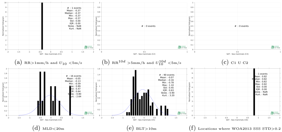
Figure 13: Normalized histogram of \Delta SSS (Aquarius-L3-JPL-V5-7DAY-RUNNING - Sea mammals) for 6 different subdatasets corresponding to: RR>1mm/h and U_{10} < 5\text{m/s} (a), RR^{10d} > 5\text{mm/h} and U_{10}^{10d} < 5\text{m/s} (b), C1 U C2 (c),MLD<20m (d),BLT>10m (e),Locations where WOA2013 SSS STD>0.2 (f).
