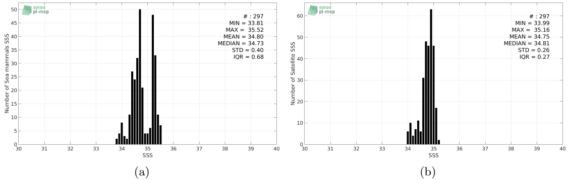
Figure 2: Histograms of SSS from Sea mammals (a) and Aquarius-L3-JPL-V5-7DAY-RUNNING (b) considering all match-up pairs per bins of 0.1 over the South Pacific Ocean Pi-MEP region and for the full satellite product period.
