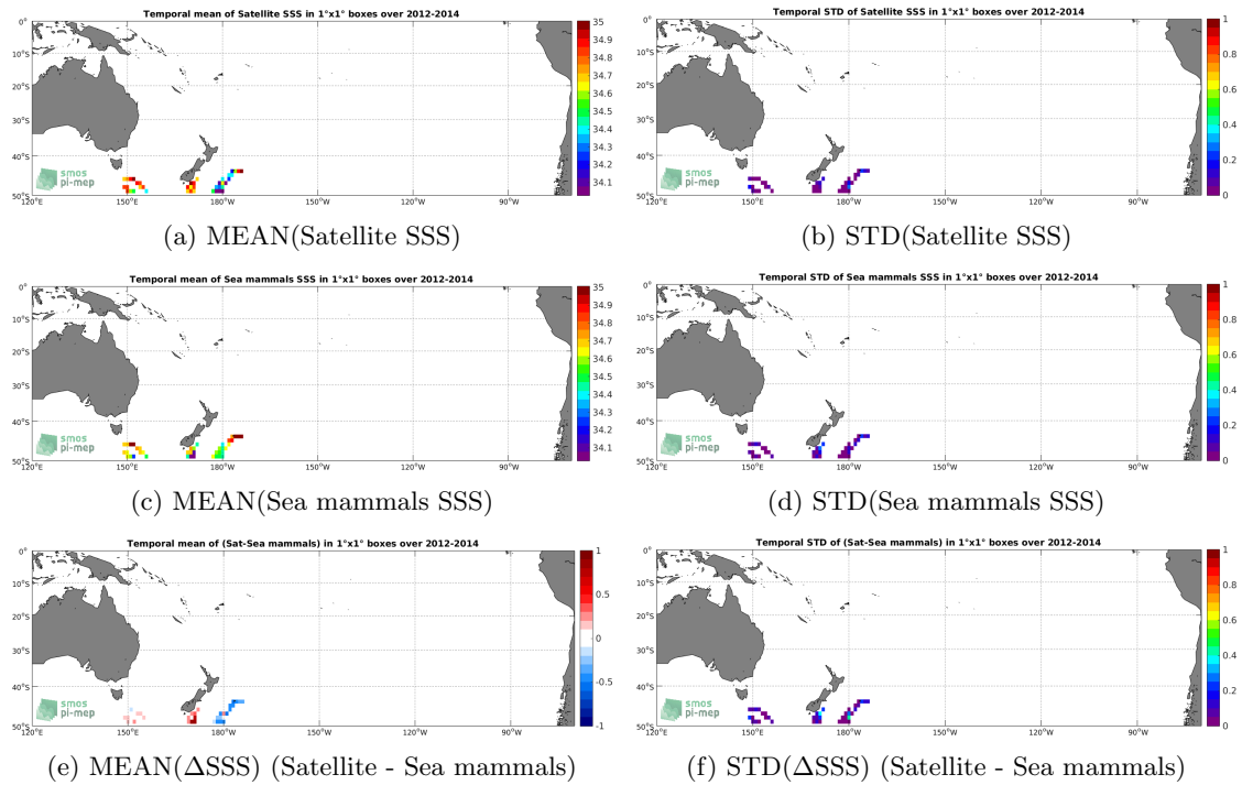
Figure 6: Temporal mean (left) and STD (right) of SSS from Aquarius-L3-JPL-V5-7DAY-RUNNING (top), Sea mammals (middle), and of \Delta SSS (Satellite - Sea mammals). Only match-up pairs are used to generate these maps.
