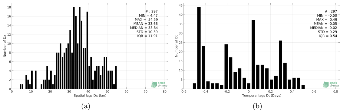
Figure 5: Histograms of the spatial (a) and temporal (b) lags between the time of the Sea mammals measurements and the date of the corresponding Aquarius-L3-JPL-V5-7DAY-RUNNING SSS product.
