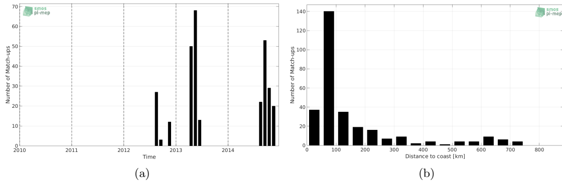
Figure 1: Number of match-ups between Sea mammals and Aquarius-L3-JPL-V5-7DAY-RUNNING SSS as a function of time (a) and as function of the distance to coast (b) over the South Pacific Ocean Pi-MEP region and for the full satellite product period.
