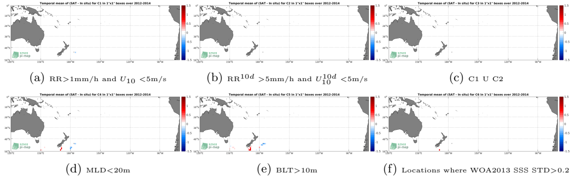
Figure 12: Temporal mean gridded over spatial boxes of size 1°x1° of \Delta SSS (Aquarius-L3-JPL-V5-7DAY-RUNNING - Sea mammals) for 6 different subdatasets corresponding to:RR>1mm/h and U_{10} < 5\text{m/s} (a), RR^{10d} > 5\text{mm/h} and U_{10}^{10d} < 5\text{m/s} (b), C1 U C2 (c),MLD<20m (d),BLT>10m (e),Locations where WOA2013 SSS STD>0.2 (f).
