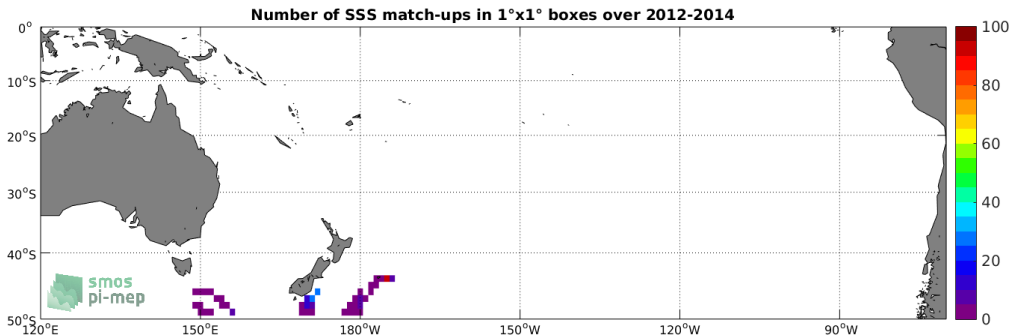
Figure 4: Number of SSS match-ups between Sea mammals SSS and the Aquarius-L3-JPL-V5-7DAY-RUNNING SSS product for the South Pacific Ocean Pi-MEP region over 1^\circ \times 1^\circ boxes and for the full satellite product period.
