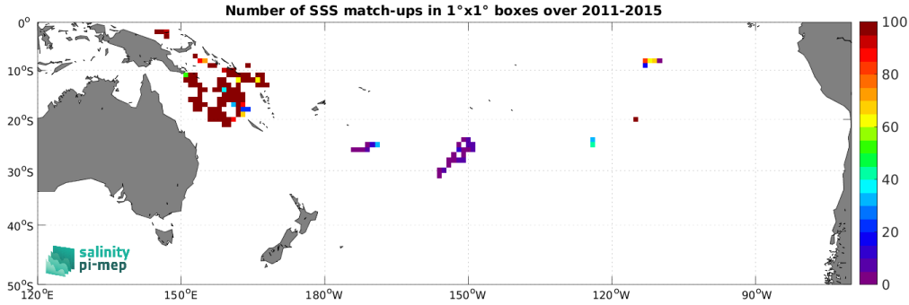
Figure 4: Number of SSS match-ups between Surface drifters SSS and the Aquarius SSS L3 CAP v5 - 7-Day running (JPL) SSS product for the South Pacific Ocean Pi-MEP region over 1^\circ \times 1^\circ boxes and for the full satellite product period.
