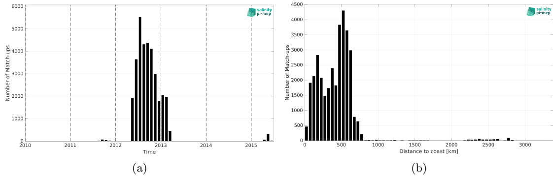
Figure 2: Number of match-ups between Surface drifters and Aquarius SSS L3 CAP v5 - 7-Day running (JPL) SSS as a function of time (a) and as function of the distance to coast (b) over the South Pacific Ocean Pi-MEP region and for the full satellite product period.
