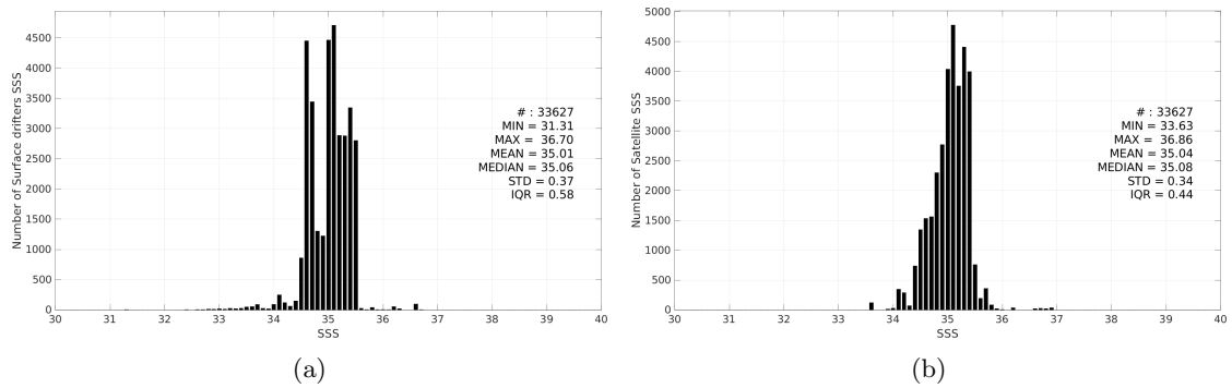
Figure 3: Histograms of SSS from Surface drifters (a) and Aquarius SSS L3 CAP v5 - 7-Day running (JPL) (b) considering all match-up pairs per bins of 0.1 over the South Pacific Ocean Pi-MEP region and for the full satellite product period.
