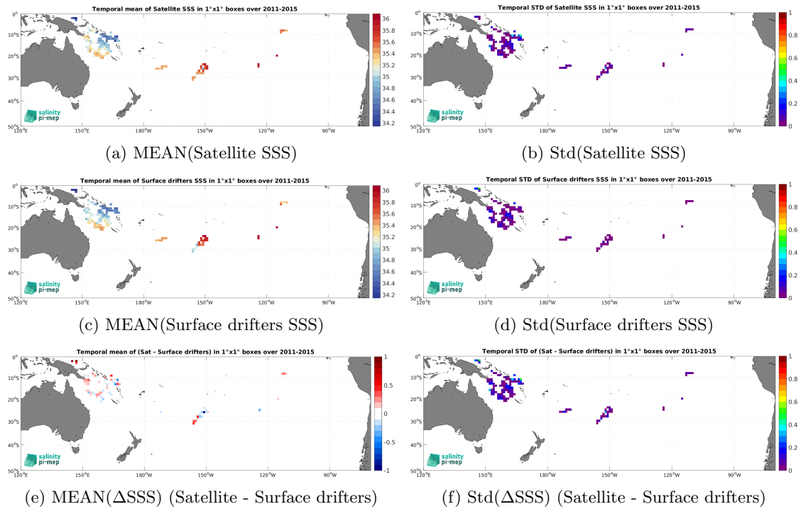
Figure 6: Temporal mean (left) and Std (right) of SSS from Aquarius SSS L3 CAP v5 - 7-Day running (JPL) (top), Surface drifters (middle), and of \Delta SSS (Satellite - Surface drifters). Only match-up pairs are used to generate these maps.
