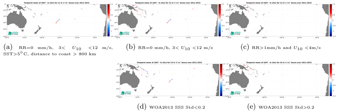
Figure 13: Temporal mean gridded over spatial boxes of size 1^\circ \times 1^\circ of \Delta SSS (Aquarius SSS L3 CAP v5 - 7-Day running (JPL) - Surface drifters) for 5 different subdatasets corresponding to:RR=0 mm/h, 3 < U_{10} < 12 m/s, SST >5^\circ C, distance to coast > 800 km (a), RR=0 mm/h, 3 < U_{10} < 12 m/s (b), RR >1 mm/h and U_{10} < 4 m/s (c), WOA2013 SSS Std <0.2 (d), WOA2013 SSS Std >0.2 (e).
