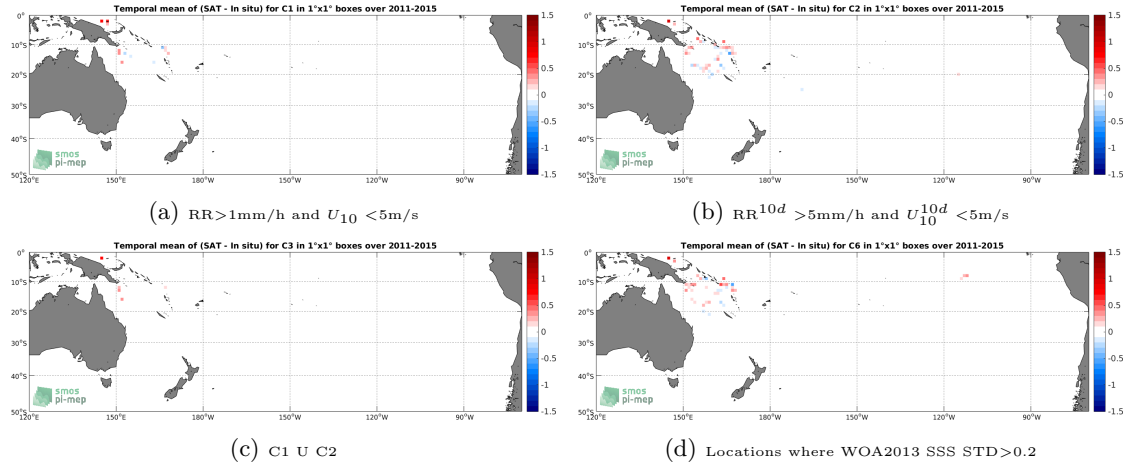
Figure 11: Temporal mean gridded over spatial boxes of size 1^\circ \times 1^\circ of \Delta SSS (Aquarius-L3-JPL-V5-7DAY-RUNNING - Surface drifters) for 4 different subdatasets corresponding to: RR > 1\text{mm/h} and U_{10} < 5\text{m/s} (a), RR^{10d} > 5\text{mm/h} and U_{10}^{10d} < 5\text{m/s} (b), C1 U C2 (c), Locations where WOA2013 SSS STD > 0.2 (d).
