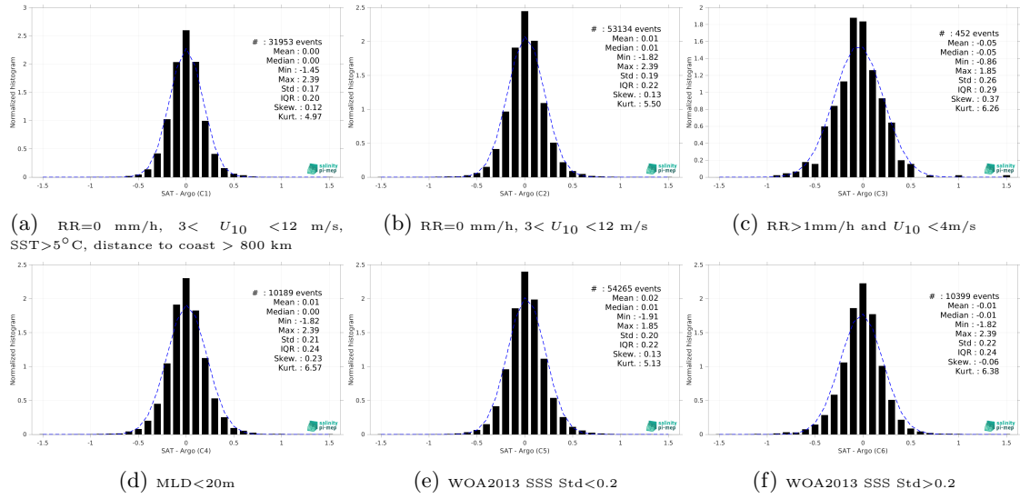
Figure 15: Normalized histogram of \Delta\text{SSS} (Aquarius SSS L3 CAP v5 - 7-Day running (JPL) - Argo) for 6 different subdatasets corresponding to: RR=0 mm/h, 3 < U_{10} < 12 m/s, SST>5°C, distance to coast > 800 km (a), RR=0 mm/h, 3 < U_{10} < 12 m/s (b), RR>1mm/h and U_{10} < 4 m/s (c), MLD<20m (d), WOA2013 SSS Std<0.2 (e), WOA2013 SSS Std>0.2 (f).
