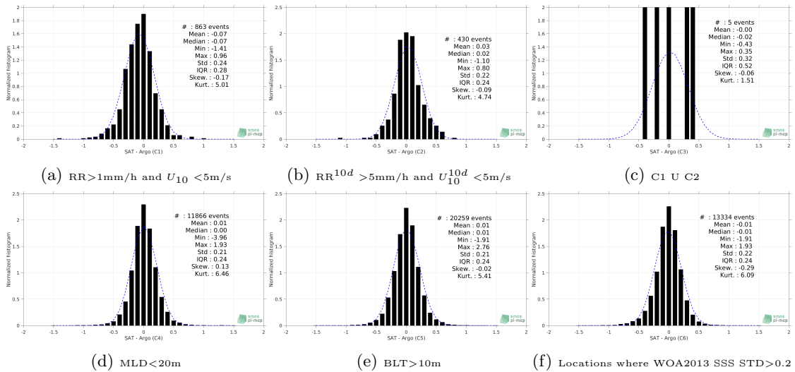
Figure 13: Normalized histogram of ΔSSS (Aquarius-L3-JPL-V5-7DAY-RUNNING - Argo) for 6 different subdatasets corresponding to: RR>1mm/h and U_{10} < 5\text{m/s} (a), RR^{10d} > 5\text{mm/h} and U_{10}^{10d} < 5\text{m/s} (b), C1 U C2 (c),MLD<20m (d),BLT>10m (e),Locations where WOA2013 SSS STD>0.2 (f).
