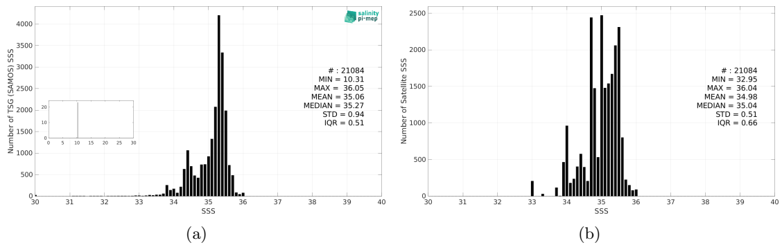
Figure 3: Histograms of SSS from TSG (SAMOS) (a) and Aquarius SSS L3 CAP v5 - Monthly (JPL) (b) considering all match-up pairs per bins of 0.1 over the South Pacific Ocean Pi-MEP region and for the full satellite product period.
