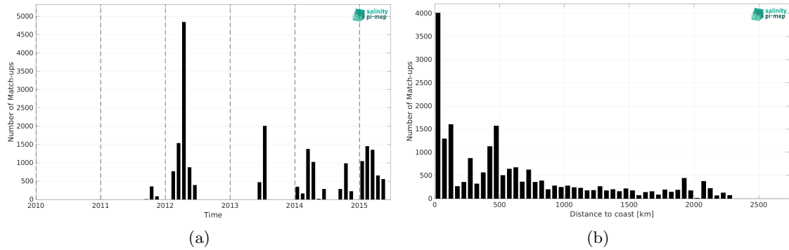
Figure 2: Number of match-ups between TSG (SAMOS) and Aquarius SSS L3 CAP v5 - Monthly (JPL) SSS as a function of time (a) and as function of the distance to coast (b) over the South Pacific Ocean Pi-MEP region and for the full satellite product period.
