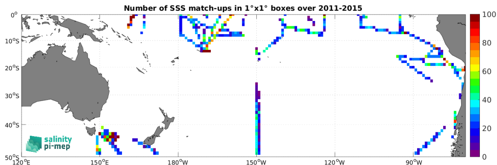
Figure 5: Number of SSS match-ups between TSG (SAMOS) SSS and the Aquarius SSS L3 CAP v5 - Monthly (JPL) SSS product for the South Pacific Ocean Pi-MEP region over 1^\circ \times 1^\circ boxes and for the full satellite product period.
