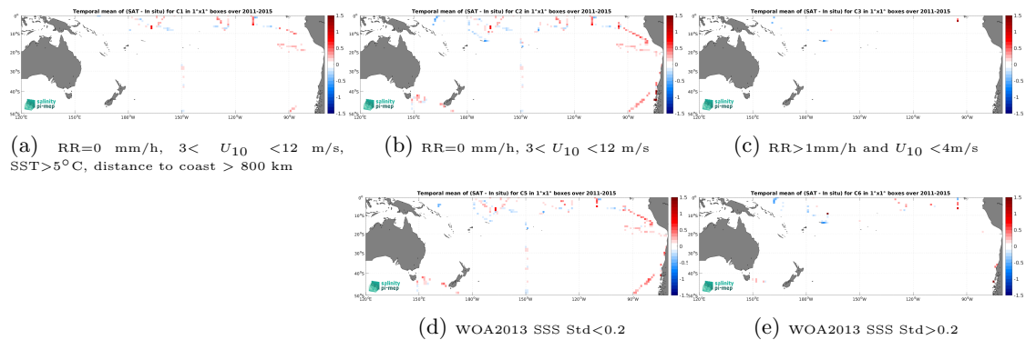
Figure 14: Temporal mean gridded over spatial boxes of size 1^\circ \times 1^\circ of \Delta SSS (Aquarius SSS L3 CAP v5 - Monthly (JPL) - TSG (SAMOS)) for 5 different subdatasets corresponding to:RR=0 mm/h, 3 < U_{10} < 12 m/s, SST >5^\circ\text{C} , distance to coast > 800 km (a), RR=0 mm/h, 3 < U_{10} < 12 m/s (b), RR >1 mm/h and U_{10} < 4 m/s (c), WOA2013 SSS Std <0.2 (d), WOA2013 SSS Std >0.2 (e).
