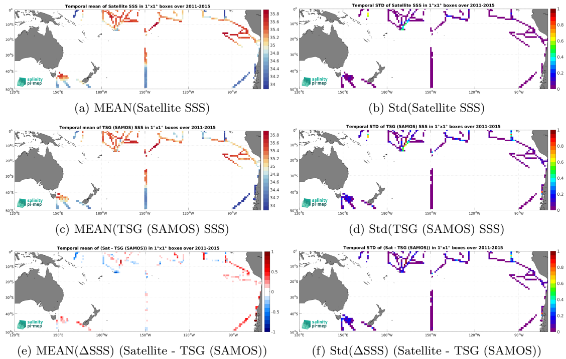
Figure 7: Temporal mean (left) and Std (right) of SSS from Aquarius SSS L3 CAP v5 - Monthly (JPL) (top), TSG (SAMOS) (middle), and of \Delta SSS (Satellite - TSG (SAMOS)). Only match-up pairs are used to generate these maps.
