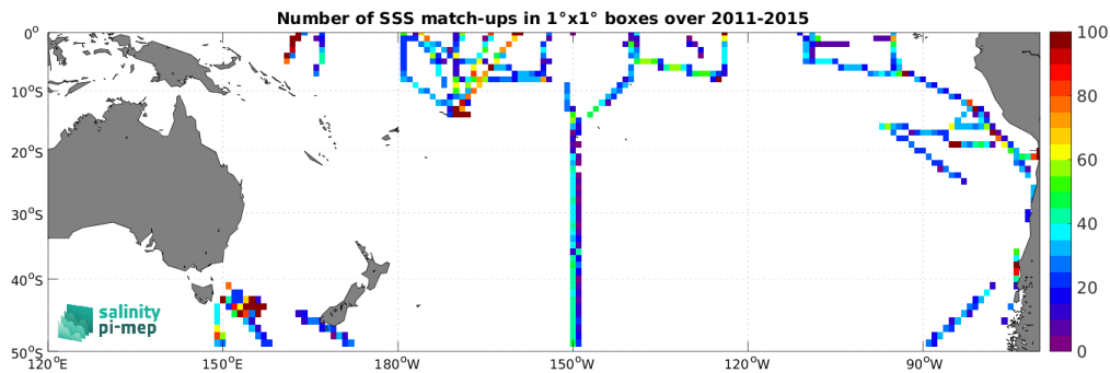
Figure 4: Number of SSS match-ups between TSG (SAMOS) SSS and the Aquarius SSS L3 CAP v5 - Monthly (JPL) SSS product for the South Pacific Ocean Pi-MEP region over 1^\circ \times 1^\circ boxes and for the full satellite product period.
