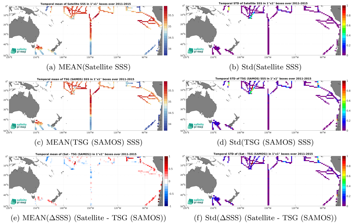
Figure 6: Temporal mean (left) and Std (right) of SSS from Aquarius SSS L3 CAP v5 - Monthly (JPL) (top), TSG (SAMOS) (middle), and of \Delta SSS (Satellite - TSG (SAMOS)). Only match-up pairs are used to generate these maps.
