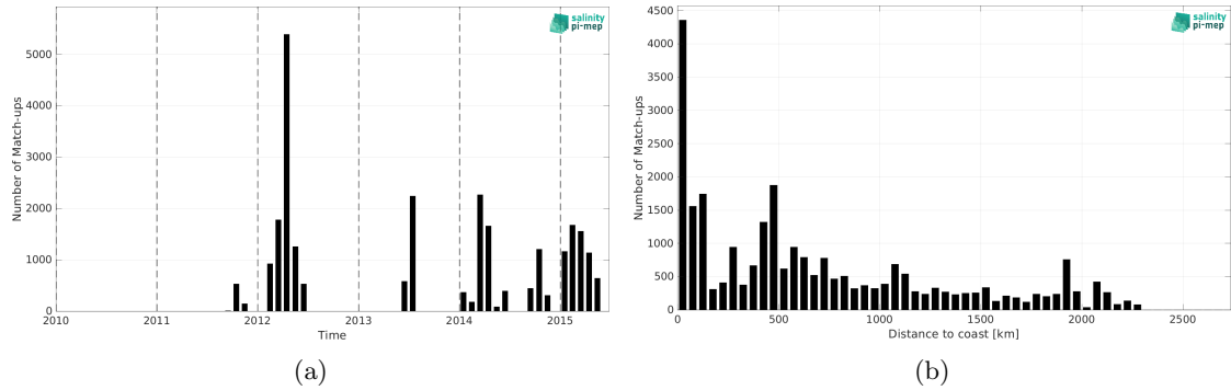
Figure 1: Number of match-ups between TSG (SAMOS) and Aquarius SSS L3 CAP v5 - Monthly (JPL) SSS as a function of time (a) and as function of the distance to coast (b) over the South Pacific Ocean Pi-MEP region and for the full satellite product period.
