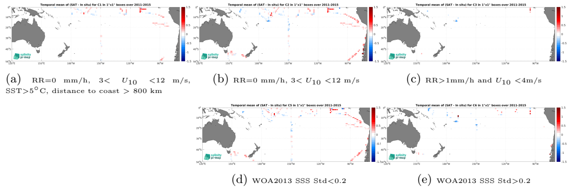
Figure 12: Temporal mean gridded over spatial boxes of size 1^\circ \times 1^\circ of \Delta SSS (Aquarius SSS L3 CAP v5 - Monthly (JPL) - TSG (SAMOS)) for 5 different subdatasets corresponding to:RR=0 mm/h, 3 < U_{10} < 12 m/s, SST >5^\circ C, distance to coast > 800 km (a), RR=0 mm/h, 3 < U_{10} < 12 m/s (b), RR >1 mm/h and U_{10} < 4 m/s (c), WOA2013 SSS Std <0.2 (d), WOA2013 SSS Std >0.2 (e).
