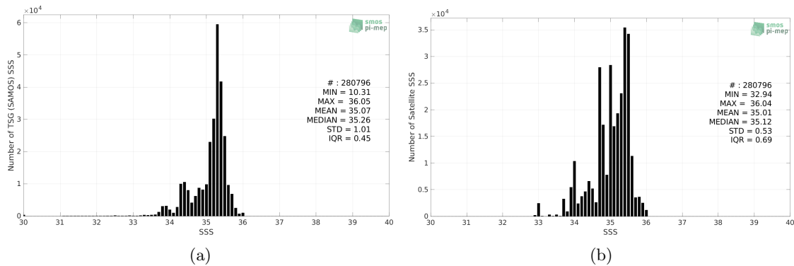
Figure 2: Histograms of SSS from TSG (SAMOS) (a) and Aquarius SSS L3 CAP v5 - Monthly (JPL) (b) considering all match-up pairs per bins of 0.1 over the South Pacific Ocean Pi-MEP region and for the full satellite product period.
