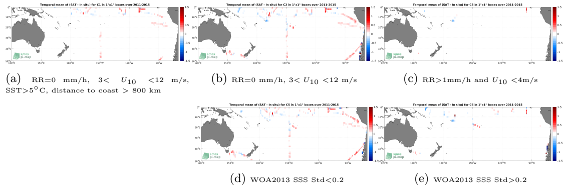
Figure 12: Temporal mean gridded over spatial boxes of size 1^\circ \times 1^\circ of \Delta\text{SSS} (Aquarius SSS L3 CAP v5 - Monthly (JPL) - TSG (SAMOS)) for 5 different subdatasets corresponding to:RR=0 mm/h, 3 < U_{10} < 12 m/s, SST >5^\circ\text{C} , distance to coast > 800 km (a), RR=0 mm/h, 3 < U_{10} < 12 m/s (b), RR >1 mm/h and U_{10} < 4 m/s (c), WOA2013 SSS Std <0.2 (d), WOA2013 SSS Std >0.2 (e).
