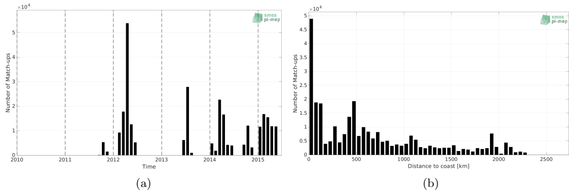
Figure 1: Number of match-ups between TSG (SAMOS) and Aquarius SSS L3 CAP v5 - Monthly (JPL) SSS as a function of time (a) and as function of the distance to coast (b) over the South Pacific Ocean Pi-MEP region and for the full satellite product period.
