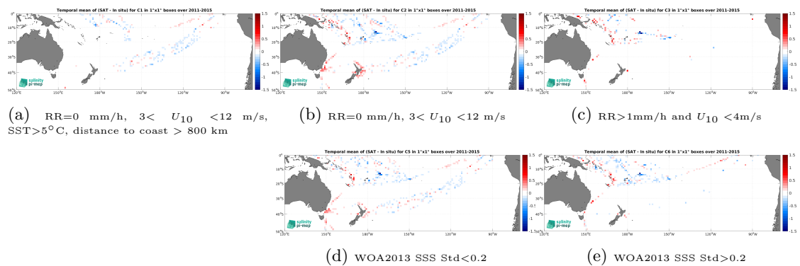
Figure 14: Temporal mean gridded over spatial boxes of size 1^\circ \times 1^\circ of \Delta SSS (Aquarius SSS L3 CAP v5 - Monthly (JPL) - TSG (LEGOS-DM)) for 5 different subdatasets corresponding to:RR=0 mm/h, 3 < U_{10} < 12 m/s, SST>5°C, distance to coast > 800 km (a), RR=0 mm/h, 3 < U_{10} < 12 m/s (b), RR>1mm/h and U_{10} < 4 m/s (c), WOA2013 SSS Std<0.2 (d), WOA2013 SSS Std>0.2 (e).
