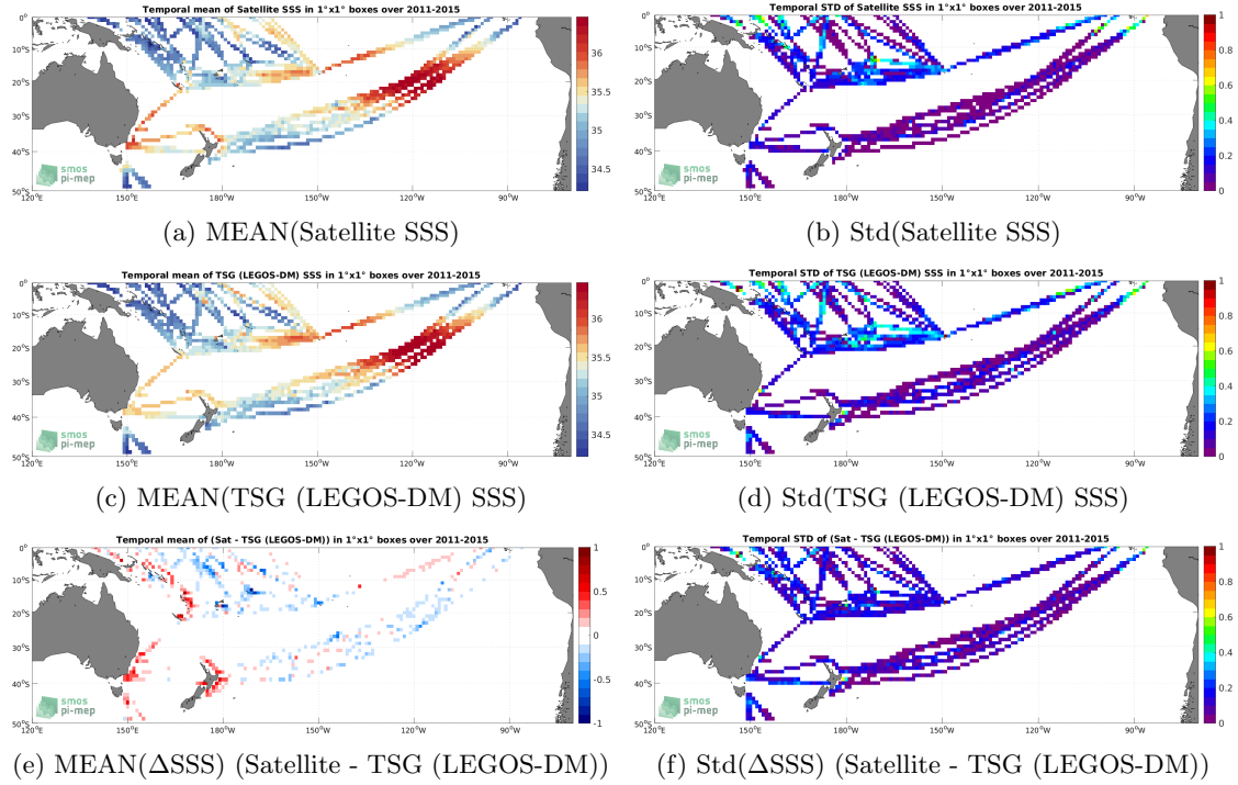
(a) MEAN(Satellite SSS) (b) Std(Satellite SSS) (c) MEAN(TSG (LEGOS-DM) SSS) (d) Std(TSG (LEGOS-DM) SSS) (e) MEAN( \Delta SSS) (Satellite - TSG (LEGOS-DM)) (f) Std( \Delta SSS) (Satellite - TSG (LEGOS-DM)) Figure 6: Temporal mean (left) and Std (right) of SSS from Aquarius SSS L3 CAP v5 - Monthly (JPL) (top), TSG (LEGOS-DM) (middle), and of \Delta SSS (Satellite - TSG (LEGOS-DM)). Only match-up pairs are used to generate these maps.
