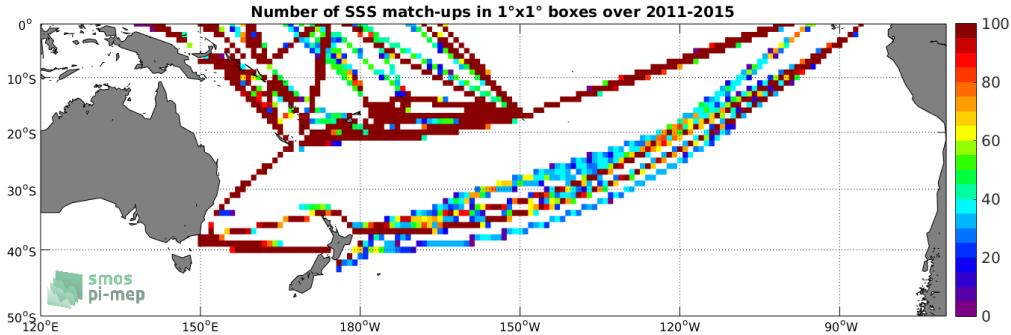
Figure 4: Number of SSS match-ups between TSG-LEGOS-DM SSS and the Aquarius-L3-JPL-V5-MONTHLY SSS product for the South Pacific Ocean Pi-MEP region over 1^\circ \times 1^\circ boxes and for the full satellite product period.
