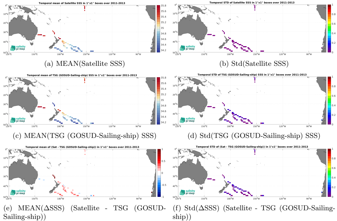
Figure 7: Temporal mean (left) and Std (right) of SSS from Aquarius SSS L3 CAP v5 - Monthly (JPL) (top), TSG (GOSUD-Sailing-ship) (middle), and of \Delta SSS (Satellite - TSG (GOSUD-Sailing-ship)). Only match-up pairs are used to generate these maps.
