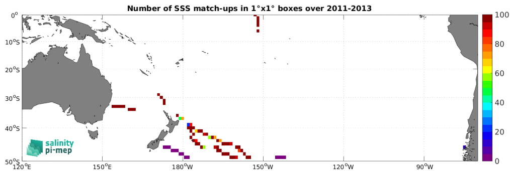
Figure 5: Number of SSS match-ups between TSG (GOSUD-Sailing-ship) SSS and the Aquarius SSS L3 CAP v5 - Monthly (JPL) SSS product for the South Pacific Ocean Pi-MEP region over 1^\circ \times 1^\circ boxes and for the full satellite product period.
