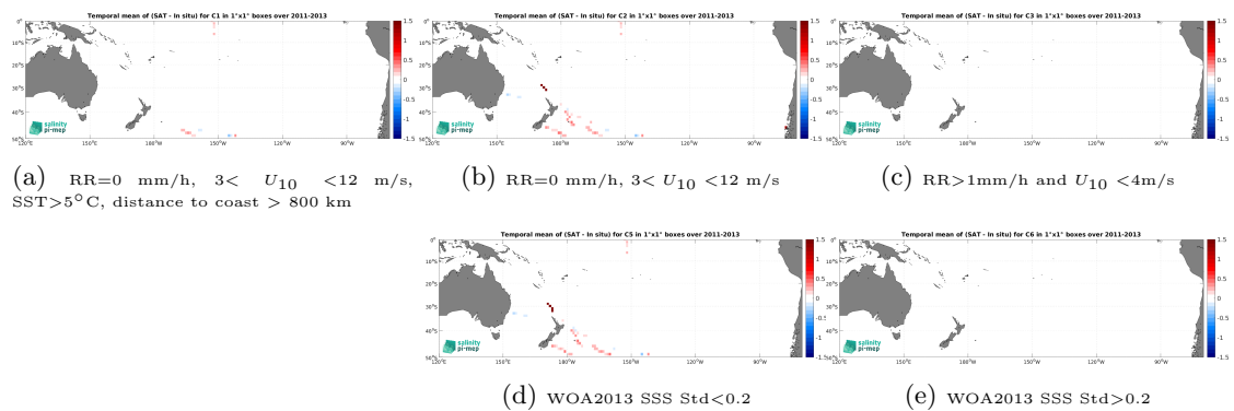
Figure 14: Temporal mean gridded over spatial boxes of size 1^\circ \times 1^\circ of \Delta SSS (Aquarius SSS L3 CAP v5 - Monthly (JPL) - TSG (GOSUD-Sailing-ship)) for 5 different subdatasets corresponding to:RR=0 mm/h, 3 < U_{10} < 12 m/s, SST >5^\circ\text{C} , distance to coast > 800 km (a), RR=0 mm/h, 3 < U_{10} < 12 m/s (b), RR >1 mm/h and U_{10} < 4 m/s (c), WOA2013 SSS Std <0.2 (d), WOA2013 SSS Std >0.2 (e).
