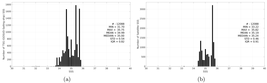
Figure 3: Histograms of SSS from TSG (GOSUD-Sailing-ship) (a) and Aquarius SSS L3 CAP v5 - Monthly (JPL) (b) considering all match-up pairs per bins of 0.1 over the South Pacific Ocean Pi-MEP region and for the full satellite product period.
