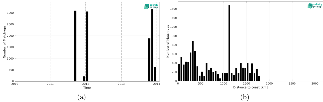
Figure 2: Number of match-ups between TSG (GOSUD-Sailing-ship) and Aquarius SSS L3 CAP v5 - Monthly (JPL) SSS as a function of time (a) and as function of the distance to coast (b) over the South Pacific Ocean Pi-MEP region and for the full satellite product period.
