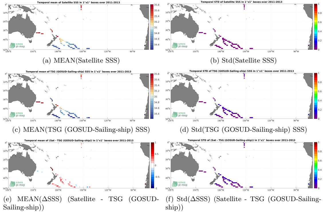
Figure 6: Temporal mean (left) and Std (right) of SSS from Aquarius SSS L3 CAP v5 - Monthly (JPL) (top), TSG (GOSUD-Sailing-ship) (middle), and of \Delta SSS (Satellite - TSG (GOSUD-Sailing-ship)). Only match-up pairs are used to generate these maps.
