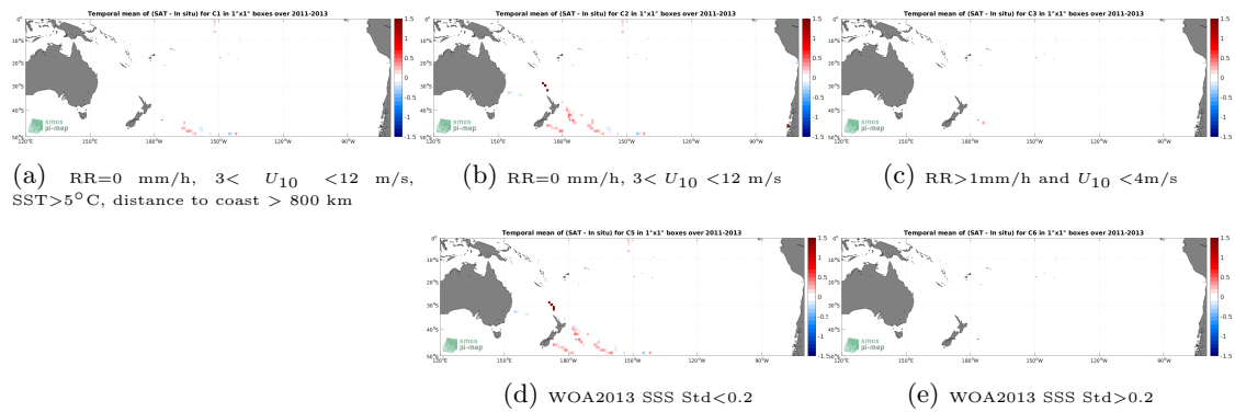
Figure 12: Temporal mean gridded over spatial boxes of size 1^\circ \times 1^\circ of \Delta\text{SSS} (Aquarius SSS L3 CAP v5 - Monthly (JPL) - TSG (GOSUD-Sailing-ship)) for 5 different subdatasets corresponding to:RR=0 mm/h, 3 < U_{10} < 12 m/s, SST>5°C, distance to coast > 800 km (a), RR=0 mm/h, 3 < U_{10} < 12 m/s (b), RR>1mm/h and U_{10} < 4 m/s (c), WOA2013 SSS Std<0.2 (d), WOA2013 SSS Std>0.2 (e).
