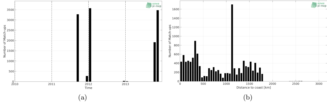
Figure 1: Number of match-ups between TSG-GOSUD-Sailing-ship and Aquarius-L3-JPL-V5-MONTHLY SSS as a function of time (a) and as function of the distance to coast (b) over the South Pacific Ocean Pi-MEP region and for the full satellite product period.
