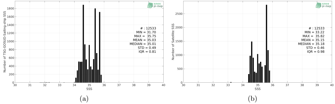
Figure 2: Histograms of SSS from TSG-GOSUD-Sailing-ship (a) and Aquarius-L3-JPL-V5-MONTHLY (b) considering all match-up pairs per bins of 0.1 over the South Pacific Ocean Pi-MEP region and for the full satellite product period.
