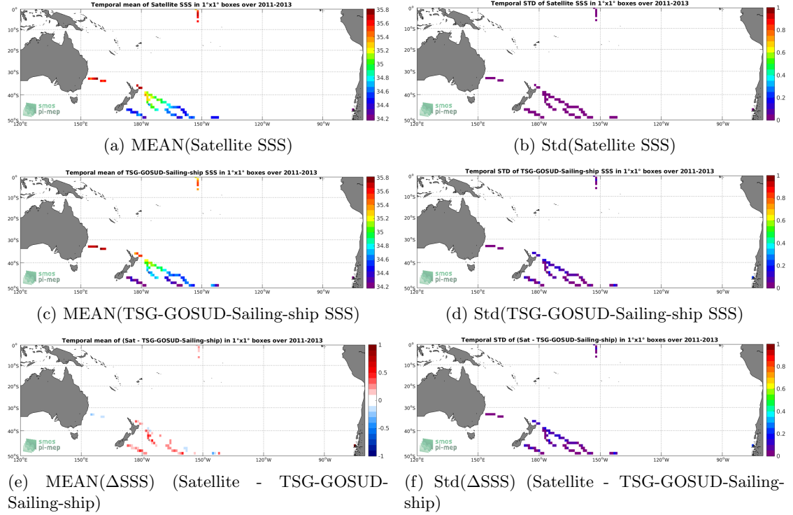
Figure 6: Temporal mean (left) and Std (right) of SSS from Aquarius-L3-JPL-V5-MONTHLY (top), TSG-GOSUD-Sailing-ship (middle), and of \Delta SSS (Satellite - TSG-GOSUD-Sailing-ship). Only match-up pairs are used to generate these maps.
