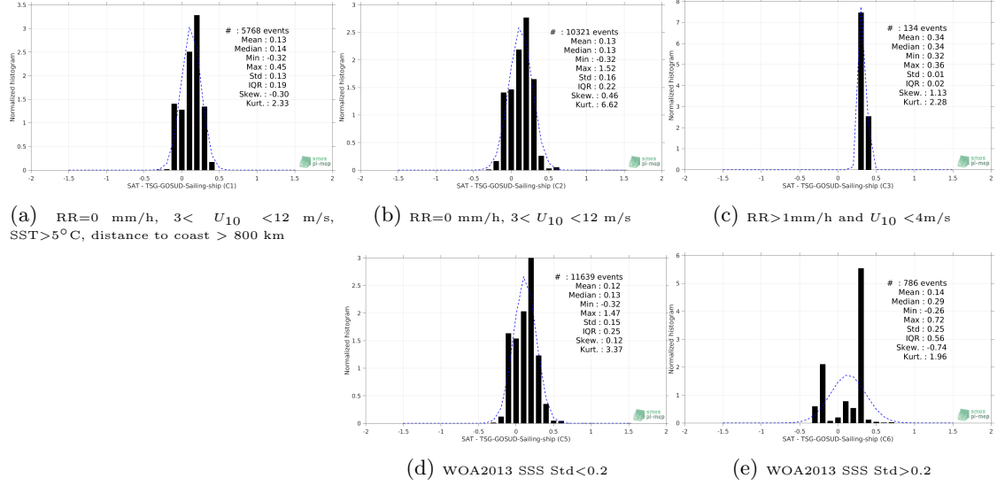
Figure 13: Normalized histogram of \Delta SSS (Aquarius-L3-JPL-V5-MONTHLY - TSG-GOSUD-Sailing-ship) for 5 different subdatasets corresponding to: RR=0 mm/h, 3 < U_{10} < 12 m/s, SST > 5^\circ\text{C} , distance to coast > 800 km (a), RR=0 mm/h, 3 < U_{10} < 12 m/s (b), RR > 1 mm/h and U_{10} < 4 m/s (c), WOA2013 SSS Std < 0.2 (d), WOA2013 SSS Std > 0.2 (e).
