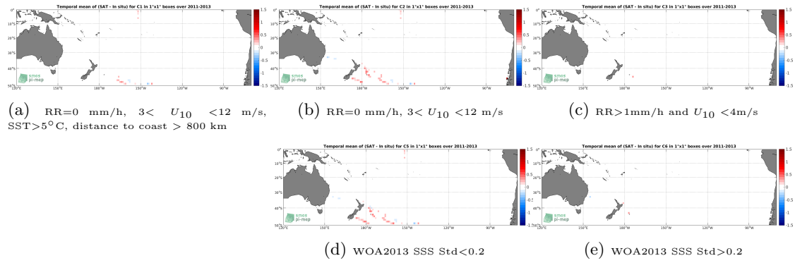
Figure 12: Temporal mean gridded over spatial boxes of size 1^\circ \times 1^\circ of \Delta SSS (Aquarius-L3-JPL-V5-MONTHLY - TSG-GOSUD-Sailing-ship) for 5 different subdatasets corresponding to: RR=0 mm/h, 3 < U_{10} < 12 m/s, SST > 5^\circ C , distance to coast > 800 km (a), RR=0 mm/h, 3 < U_{10} < 12 m/s (b), RR > 1 mm/h and U_{10} < 4 m/s (c), WOA2013 SSS Std < 0.2 (d), WOA2013 SSS Std > 0.2 (e).
