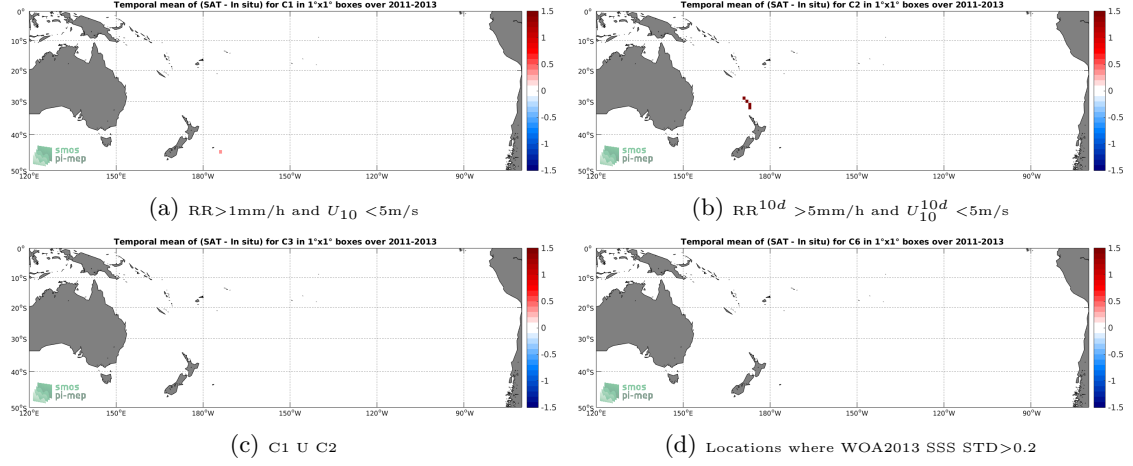
Figure 12: Temporal mean gridded over spatial boxes of size 1^\circ \times 1^\circ of \Delta SSS (Aquarius-L3-JPL-V5-MONTHLY - TSG-GOSUD-Sailing-ship) for 4 different subdatasets corresponding to: RR > 1\text{mm/h} and U_{10} < 5\text{m/s} (a), RR^{10d} > 5\text{mm/h} and U_{10}^{10d} < 5\text{m/s} (b), C1 U C2 (c), Locations where WOA2013 SSS STD > 0.2 (d).
