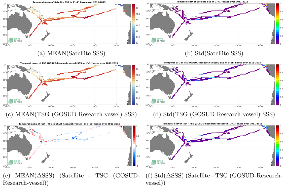
Figure 6: Temporal mean (left) and Std (right) of SSS from Aquarius SSS L3 CAP v5 - Monthly (JPL) (top), TSG (GOSUD-Research-vessel) (middle), and of \Delta SSS (Satellite - TSG (GOSUD-Research-vessel)). Only match-up pairs are used to generate these maps.
