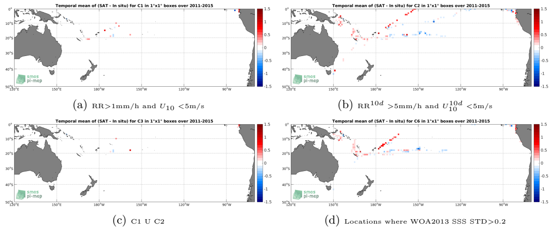
Figure 12: Temporal mean gridded over spatial boxes of size 1^\circ \times 1^\circ of \Delta SSS (Aquarius-L3-JPL-V5-MONTHLY - TSG-GOSUD-Research-vessel) for 4 different subdatasets corresponding to: RR > 1\text{mm/h} and U_{10} < 5\text{m/s} (a), RR^{10d} > 5\text{mm/h} and U_{10}^{10d} < 5\text{m/s} (b), C1 U C2 (c), Locations where WOA2013 SSS STD > 0.2 (d).
