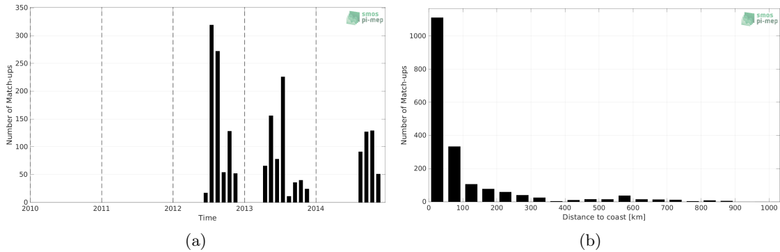
Figure 1: Number of match-ups between Marine mammals and Aquarius SSS L3 CAP v5 - Monthly (JPL) SSS as a function of time (a) and as function of the distance to coast (b) over the South Pacific Ocean Pi-MEP region and for the full satellite product period.
