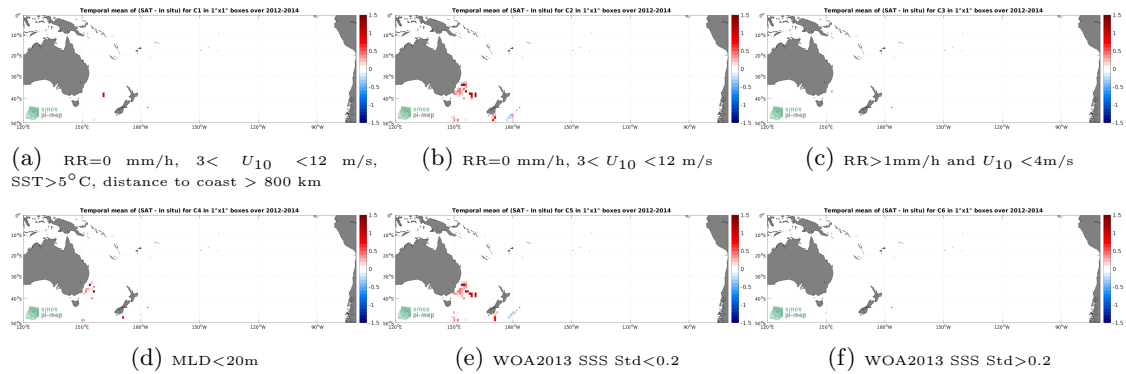
Figure 12: Temporal mean gridded over spatial boxes of size 1^\circ \times 1^\circ of \Delta SSS (Aquarius SSS L3 CAP v5 - Monthly (JPL) - Marine mammals) for 6 different subdatasets corresponding to:RR=0 mm/h, 3 < U_{10} < 12 m/s, SST >5^\circ\text{C} , distance to coast > 800 km (a), RR=0 mm/h, 3 < U_{10} < 12 m/s (b), RR >1 mm/h and U_{10} < 4 m/s (c),MLD <20 m (d),WOA2013 SSS Std <0.2 (e),WOA2013 SSS Std >0.2 (f).
