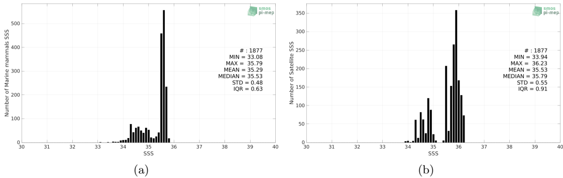
Figure 2: Histograms of SSS from Marine mammals (a) and Aquarius SSS L3 CAP v5 - Monthly (JPL) (b) considering all match-up pairs per bins of 0.1 over the South Pacific Ocean Pi-MEP region and for the full satellite product period.
