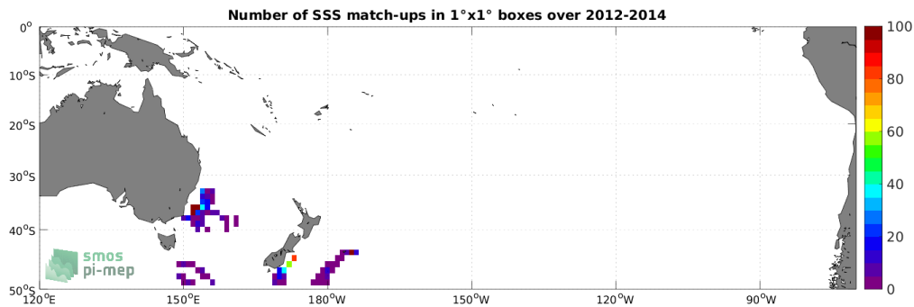
Figure 4: Number of SSS match-ups between Marine mammals SSS and the Aquarius SSS L3 CAP v5 - Monthly (JPL) SSS product for the South Pacific Ocean Pi-MEP region over 1^\circ \times 1^\circ boxes and for the full satellite product period.
