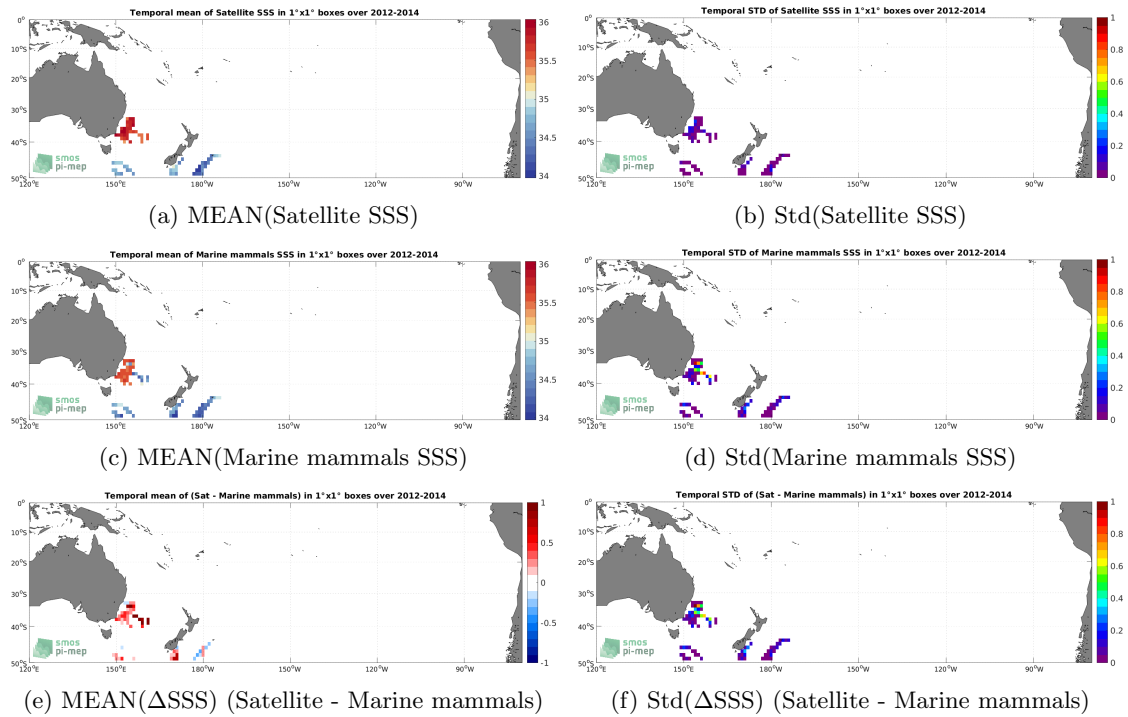
Figure 6: Temporal mean (left) and Std (right) of SSS from Aquarius SSS L3 CAP v5 - Monthly (JPL) (top), Marine mammals (middle), and of \Delta SSS (Satellite - Marine mammals). Only match-up pairs are used to generate these maps.
