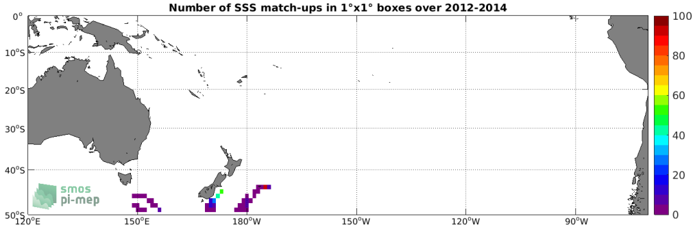
Figure 4: Number of SSS match-ups between Sea mammals SSS and the Aquarius SSS L3 CAP v5 - Monthly (JPL) SSS product for the South Pacific Ocean Pi-MEP region over 1^\circ \times 1^\circ boxes and for the full satellite product period.
