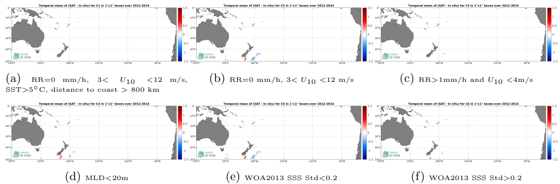
Figure 12: Temporal mean gridded over spatial boxes of size 1^{\circ}\times 1^{\circ} of \Delta\text{SSS} (Aquarius SSS L3 CAP v5 - Monthly (JPL) - Sea mammals) for 6 different subdatasets corresponding to: \text{RR}=0 mm/h, 3 < U_{10} < 12 m/s, \text{SST} > 5^{\circ}\text{C} , distance to coast > 800 km (a), \text{RR}=0 mm/h, 3 < U_{10} < 12 m/s (b), \text{RR} > 1\text{mm/h} and U_{10} < 4\text{m/s} (c), \text{MLD} < 20\text{m} (d), \text{WOA2013 SSS Std} < 0.2 (e), \text{WOA2013 SSS Std} > 0.2 (f).
