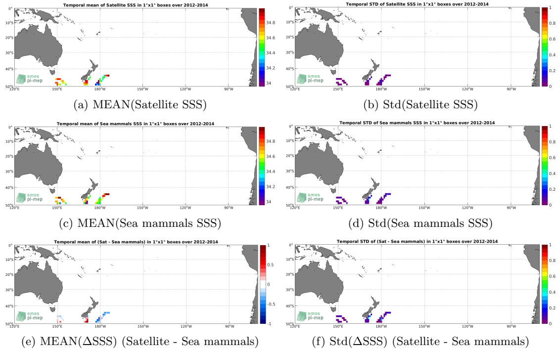
Figure 6: Temporal mean (left) and Std (right) of SSS from Aquarius SSS L3 CAP v5 - Monthly (JPL) (top), Sea mammals (middle), and of \Delta SSS (Satellite - Sea mammals). Only match-up pairs are used to generate these maps.
