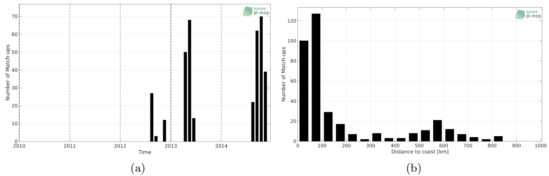
Figure 1: Number of match-ups between Sea mammals and Aquarius SSS L3 CAP v5 - Monthly (JPL) SSS as a function of time (a) and as function of the distance to coast (b) over the South Pacific Ocean Pi-MEP region and for the full satellite product period.
