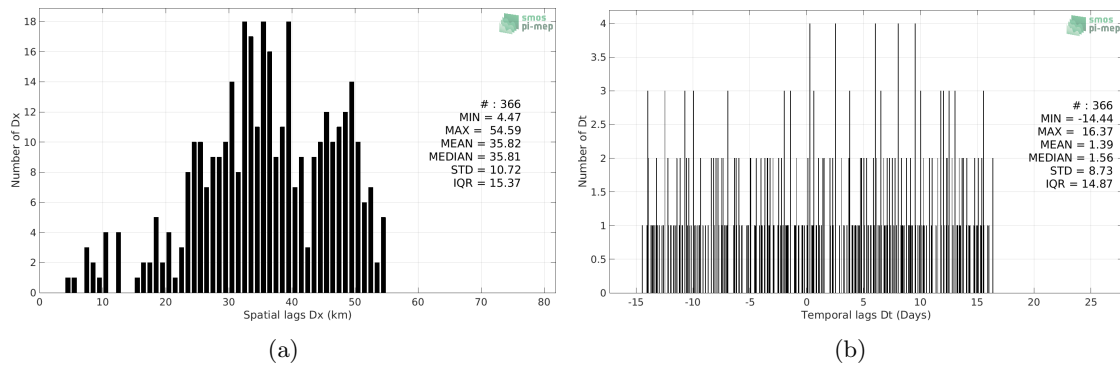
Figure 5: Histograms of the spatial (a) and temporal (b) lags between the time of the Sea mammals measurements and the date of the corresponding Aquarius SSS L3 CAP v5 - Monthly (JPL) SSS product.
