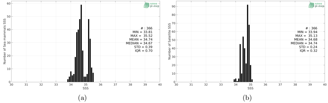
Figure 2: Histograms of SSS from Sea mammals (a) and Aquarius SSS L3 CAP v5 - Monthly (JPL) (b) considering all match-up pairs per bins of 0.1 over the South Pacific Ocean Pi-MEP region and for the full satellite product period.
