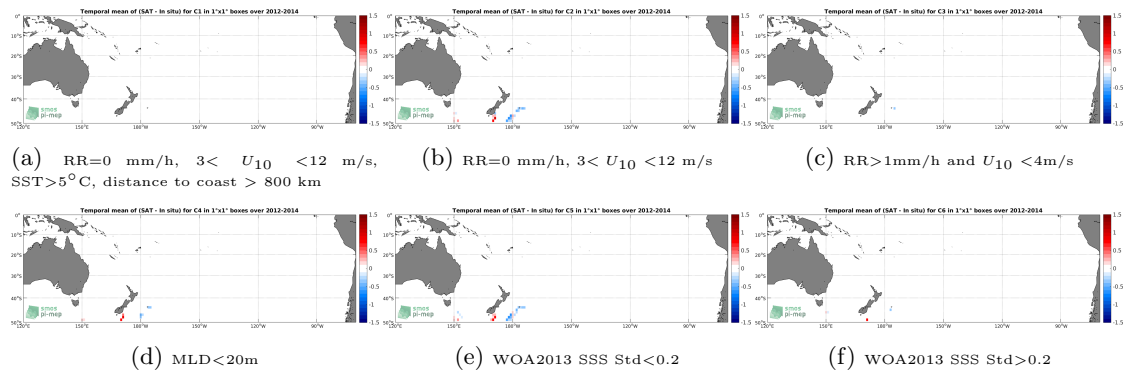
Figure 12: Temporal mean gridded over spatial boxes of size 1^{\circ}\times 1^{\circ} of \Delta\text{SSS} (Aquarius-L3-JPL-V5-MONTHLY - Sea mammals) for 6 different subdatasets corresponding to: \text{RR}=0 mm/h, 3 < U_{10} < 12 m/s, \text{SST} > 5^{\circ}\text{C} , distance to coast > 800 km (a), \text{RR}=0 mm/h, 3 < U_{10} < 12 m/s (b), \text{RR} > 1\text{mm/h} and U_{10} < 4\text{m/s} (c), \text{MLD} < 20\text{m} (d), \text{WOA2013 SSS Std} < 0.2 (e), \text{WOA2013 SSS Std} > 0.2 (f).
