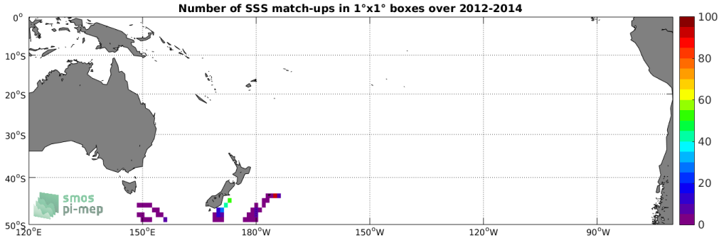
Figure 4: Number of SSS match-ups between Sea mammals SSS and the Aquarius-L3-JPL-V5-MONTHLY SSS product for the South Pacific Ocean Pi-MEP region over 1^\circ \times 1^\circ boxes and for the full satellite product period.
