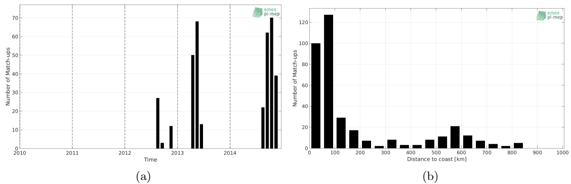
Figure 1: Number of match-ups between Sea mammals and Aquarius-L3-JPL-V5-MONTHLY SSS as a function of time (a) and as function of the distance to coast (b) over the South Pacific Ocean Pi-MEP region and for the full satellite product period.
