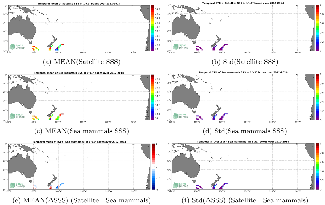
Figure 6: Temporal mean (left) and Std (right) of SSS from Aquarius-L3-JPL-V5-MONTHLY (top), Sea mammals (middle), and of \Delta SSS (Satellite - Sea mammals). Only match-up pairs are used to generate these maps.
