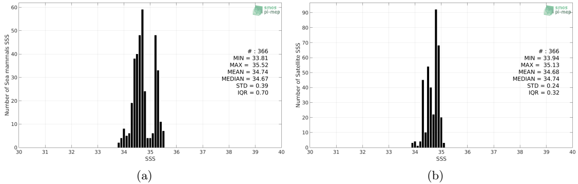
Figure 2: Histograms of SSS from Sea mammals (a) and Aquarius-L3-JPL-V5-MONTHLY (b) considering all match-up pairs per bins of 0.1 over the South Pacific Ocean Pi-MEP region and for the full satellite product period.
