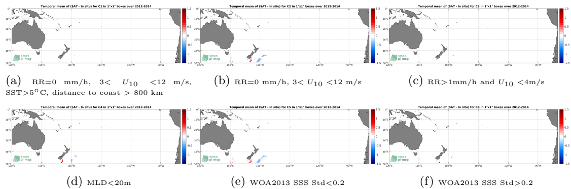
Figure 12: Temporal mean gridded over spatial boxes of size 1^\circ \times 1^\circ of \Delta SSS (Aquarius-L3-JPL-V5-MONTHLY - Sea mammals) for 6 different subdatasets corresponding to:RR=0 mm/h, 3 < U_{10} < 12 m/s, SST > 5^\circ\text{C} , distance to coast > 800 km (a), RR=0 mm/h, 3 < U_{10} < 12 m/s (b), RR > 1 mm/h and U_{10} < 4 m/s (c),MLD < 20 m (d),WOA2013 SSS Std < 0.2 (e),WOA2013 SSS Std > 0.2 (f).
