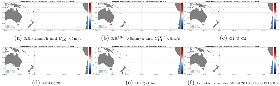
Figure 12: Temporal mean gridded over spatial boxes of size 1°x1° of \Delta SSS (Aquarius-L3-JPL-V5-MONTHLY - Sea mammals) for 6 different subdatasets corresponding to:RR>1mm/h and U_{10} < 5m/s (a), RR^{10d} > 5mm/h and U_{10}^{10d} < 5m/s (b), C1 U C2 (c),MLD<20m (d),BLT>10m (e),Locations where WOA2013 SSS STD>0.2 (f).
