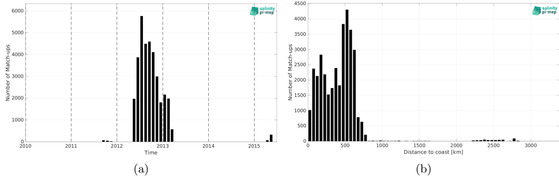
Figure 2: Number of match-ups between Surface drifters and Aquarius SSS L3 CAP v5 - Monthly (JPL) SSS as a function of time (a) and as function of the distance to coast (b) over the South Pacific Ocean Pi-MEP region and for the full satellite product period.
