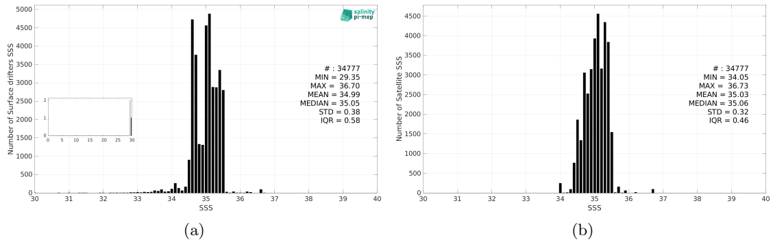
Figure 3: Histograms of SSS from Surface drifters (a) and Aquarius SSS L3 CAP v5 - Monthly (JPL) (b) considering all match-up pairs per bins of 0.1 over the South Pacific Ocean Pi-MEP region and for the full satellite product period.
