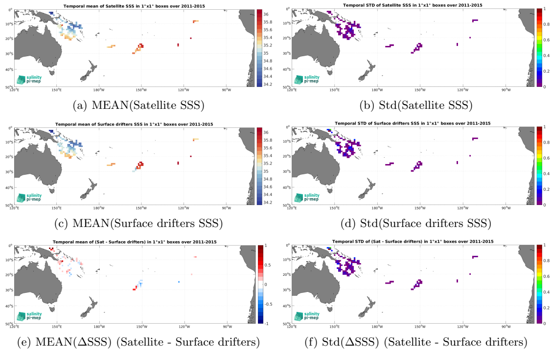
Figure 6: Temporal mean (left) and Std (right) of SSS from Aquarius SSS L3 CAP v5 - Monthly (JPL) (top), Surface drifters (middle), and of \Delta SSS (Satellite - Surface drifters). Only match-up pairs are used to generate these maps.
