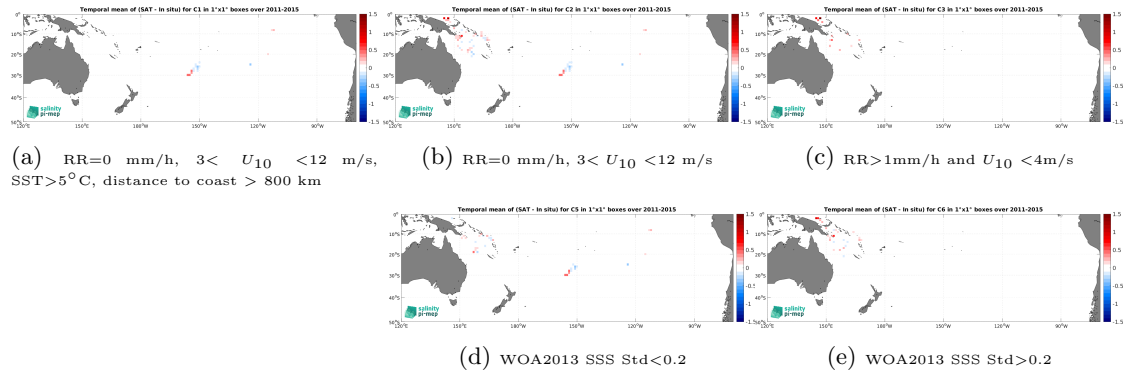
Figure 13: Temporal mean gridded over spatial boxes of size 1^\circ \times 1^\circ of \Delta SSS (Aquarius SSS L3 CAP v5 - Monthly (JPL) - Surface drifters) for 5 different subdatasets corresponding to:RR=0 mm/h, 3 < U_{10} < 12 m/s, SST >5^\circ\text{C} , distance to coast > 800 km (a), RR=0 mm/h, 3 < U_{10} < 12 m/s (b), RR >1 mm/h and U_{10} < 4 m/s (c), WOA2013 SSS Std <0.2 (d), WOA2013 SSS Std >0.2 (e).
