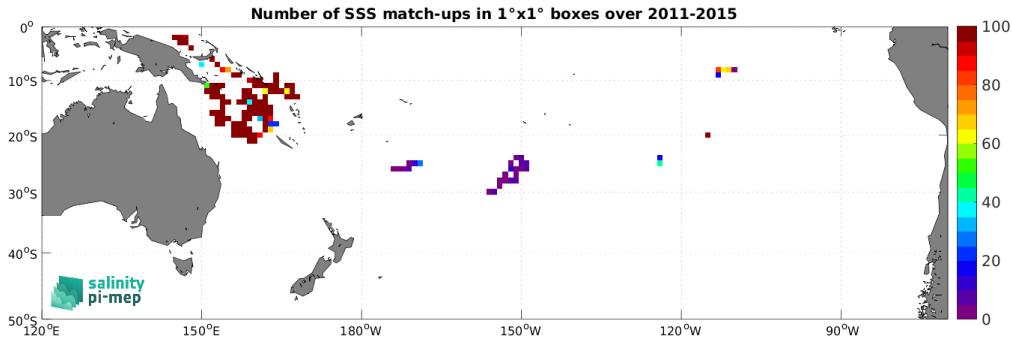
Figure 4: Number of SSS match-ups between Surface drifters SSS and the Aquarius SSS L3 CAP v5 - Monthly (JPL) SSS product for the South Pacific Ocean Pi-MEP region over 1^\circ \times 1^\circ boxes and for the full satellite product period.
