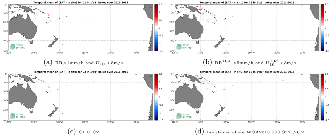
Figure 11: Temporal mean gridded over spatial boxes of size 1^\circ \times 1^\circ of \Delta SSS (Aquarius-L3-JPL-V5-MONTHLY - Surface drifters) for 4 different subdatasets corresponding to:RR >1 mm/h and U_{10} < 5 m/s (a), RR^{10d} > 5 mm/h and U_{10}^{10d} < 5 m/s (b), C1 U C2 (c),Locations where WOA2013 SSS STD >0.2 (d).
