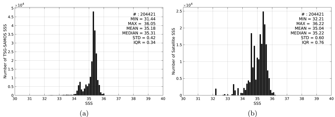
Figure 2: Histograms of SSS from TSG-SAMOS (a) and Aquarius-L3-JPL-V4-7DAY-RUNNING (b) considering all match-up pairs per bins of 0.1 over the South Pacific Ocean Pi-MEP region and for the full satellite product period.
