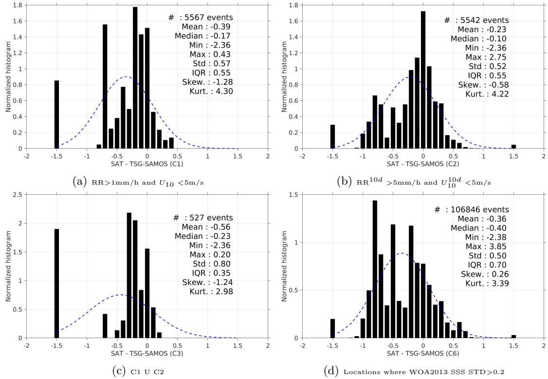
Figure 13: Normalized histogram of \Delta SSS (Aquarius-L3-JPL-V4-7DAY-RUNNING - TSG-SAMOS) for 6 different subdatasets corresponding to: RR > 1\text{mm/h} and U_{10} < 5\text{m/s} (a), RR^{10d} > 5\text{mm/h} and U_{10}^{10d} < 5\text{m/s} (b), C1 U C2 (c), Locations where WOA2013 SSS STD > 0.2 (d).
