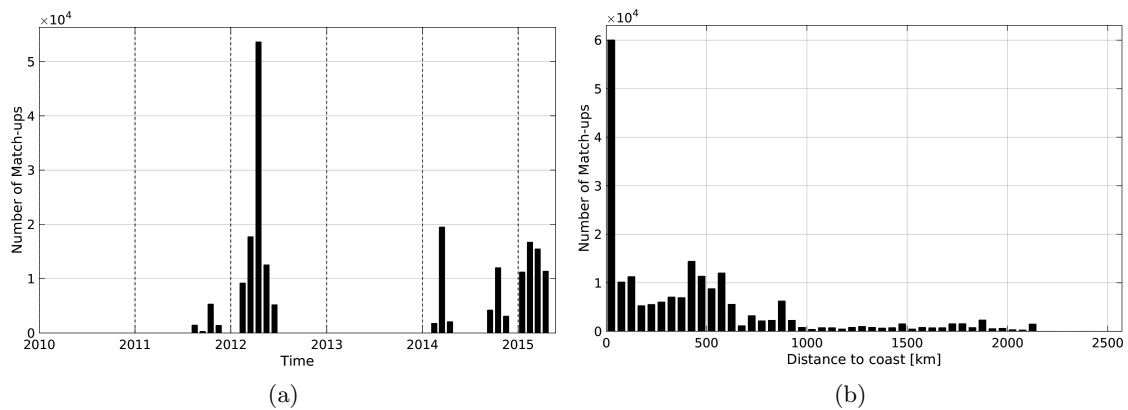
Figure 1: Number of match-ups between TSG-SAMOS and Aquarius-L3-JPL-V4-7DAY-RUNNING SSS as a function of time (a) and as function of the distance to coast (b) over the South Pacific Ocean Pi-MEP region and for the full satellite product period.
