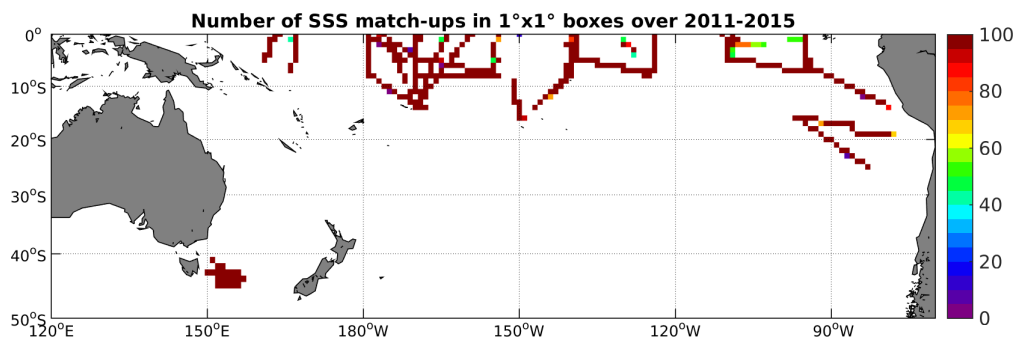
Figure 4: Number of SSS match-ups between TSG-SAMOS SSS and the Aquarius-L3-JPL-V4-7DAY-RUNNING SSS product for the South Pacific Ocean Pi-MEP region over 1^\circ \times 1^\circ boxes and for the full satellite product period.
