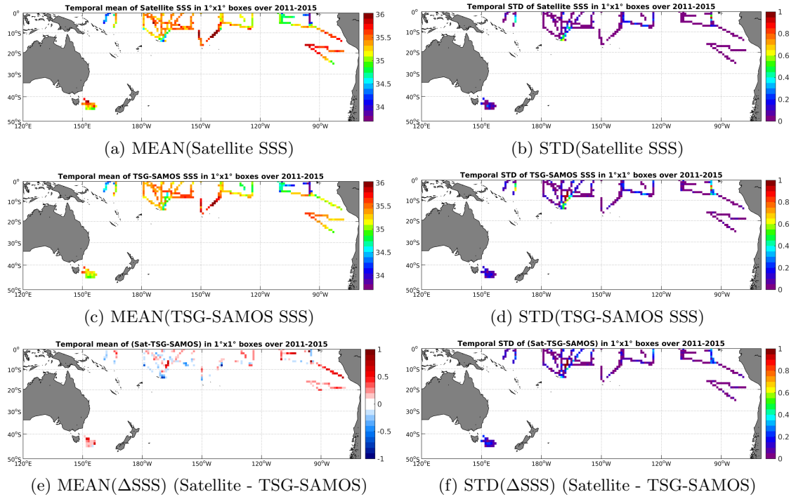
Figure 6: Temporal mean (left) and STD (right) of SSS from Aquarius-L3-JPL-V4-7DAY-RUNNING (top), TSG-SAMOS (middle), and of \Delta SSS (Satellite - TSG-SAMOS). Only match-up pairs are used to generate these maps.
