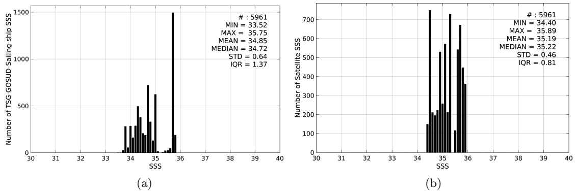
Figure 2: Histograms of SSS from TSG-GOSUD-Sailing-ship (a) and Aquarius-L3-JPL-V4-7DAY-RUNNING (b) considering all match-up pairs per bins of 0.1 over the South Pacific Ocean Pi-MEP region and for the full satellite product period.
