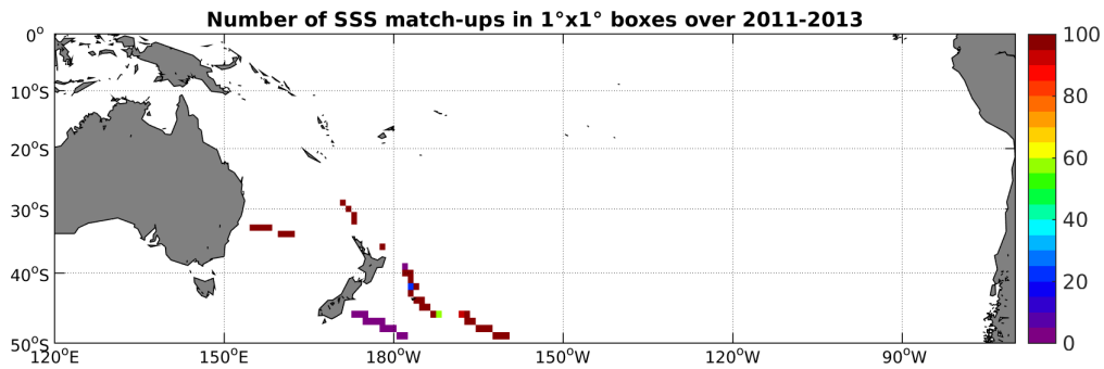
Figure 4: Number of SSS match-ups between TSG-GOSUD-Sailing-ship SSS and the Aquarius-L3-JPL-V4-7DAY-RUNNING SSS product for the South Pacific Ocean Pi-MEP region over 1^{\circ} \times 1^{\circ} boxes and for the full satellite product period.
