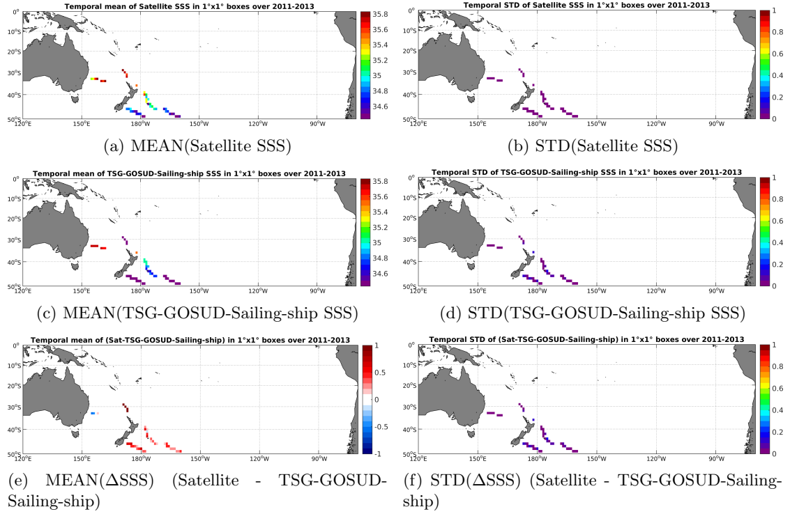
Figure 6: Temporal mean (left) and STD (right) of SSS from Aquarius-L3-JPL-V4-7DAY-RUNNING (top), TSG-GOSUD-Sailing-ship (middle), and of \Delta SSS (Satellite - TSG-GOSUD-Sailing-ship). Only match-up pairs are used to generate these maps.
