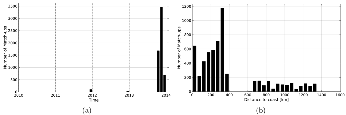
Figure 1: Number of match-ups between TSG-GOSUD-Sailing-ship and Aquarius-L3-JPL-V4-7DAY-RUNNING SSS as a function of time (a) and as function of the distance to coast (b) over the South Pacific Ocean Pi-MEP region and for the full satellite product period.
