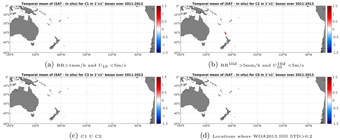
Figure 12: Temporal mean gridded over spatial boxes of size 1^\circ \times 1^\circ of \Delta SSS (Aquarius-L3-JPL-V4-7DAY-RUNNING - TSG-GOSUD-Sailing-ship) for 4 different subdatasets corresponding to: RR > 1 mm/h and U_{10} < 5 m/s (a), RR 10d > 5 mm/h and U_{10d} < 5 m/s (b), C1 U C2 (c), Locations where WOA2013 SSS STD > 0.2 (d).
