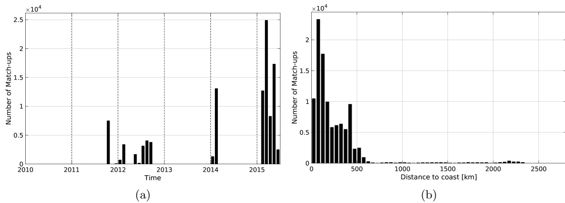
Figure 1: Number of match-ups between TSG-GOSUD-Research-vessel and Aquarius-L3-JPL-V4-7DAY-RUNNING SSS as a function of time (a) and as function of the distance to coast (b) over the South Pacific Ocean Pi-MEP region and for the full satellite product period.
