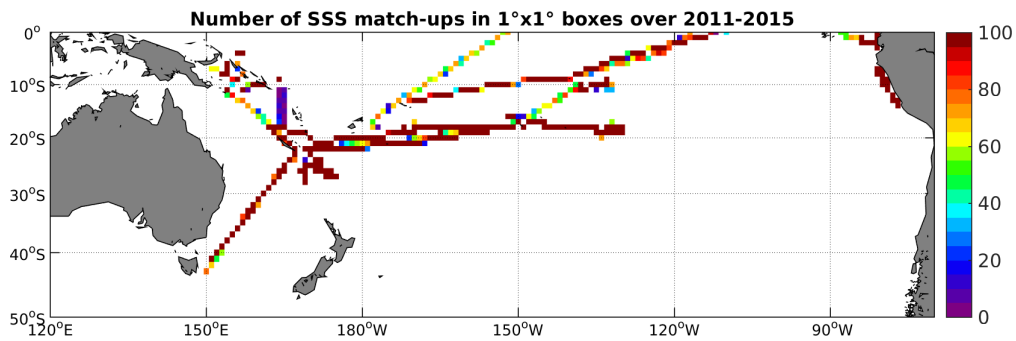
Figure 4: Number of SSS match-ups between TSG-GOSUD-Research-vessel SSS and the Aquarius-L3-JPL-V4-7DAY-RUNNING SSS product for the South Pacific Ocean Pi-MEP region over 1^\circ \times 1^\circ boxes and for the full satellite product period.
