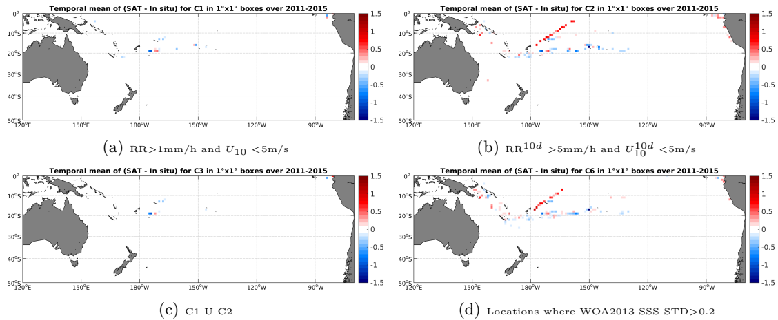
Figure 12: Temporal mean gridded over spatial boxes of size 1^\circ \times 1^\circ of \Delta SSS (Aquarius-L3-JPL-V4-7DAY-RUNNING - TSG-GOSUD-Research-vessel) for 4 different subdatasets corresponding to: RR > 1 mm/h and U_{10} < 5 m/s (a), RR 10d > 5 mm/h and U_{10}^{10d} < 5 m/s (b), C1 U C2 (c), Locations where WOA2013 SSS STD > 0.2 (d).
