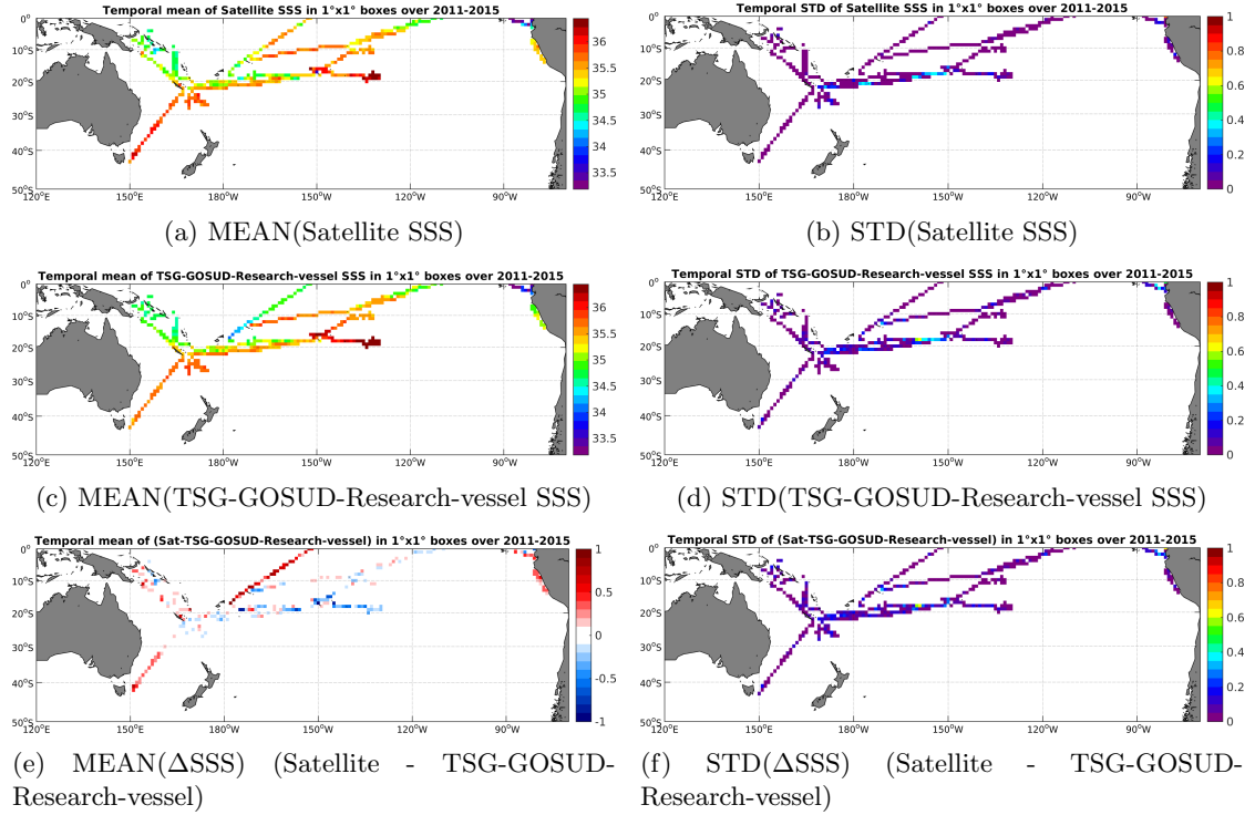
Figure 6: Temporal mean (left) and STD (right) of SSS from Aquarius-L3-JPL-V4-7DAY-RUNNING (top), TSG-GOSUD-Research-vessel (middle), and of \Delta SSS (Satellite - TSG-GOSUD-Research-vessel). Only match-up pairs are used to generate these maps.
