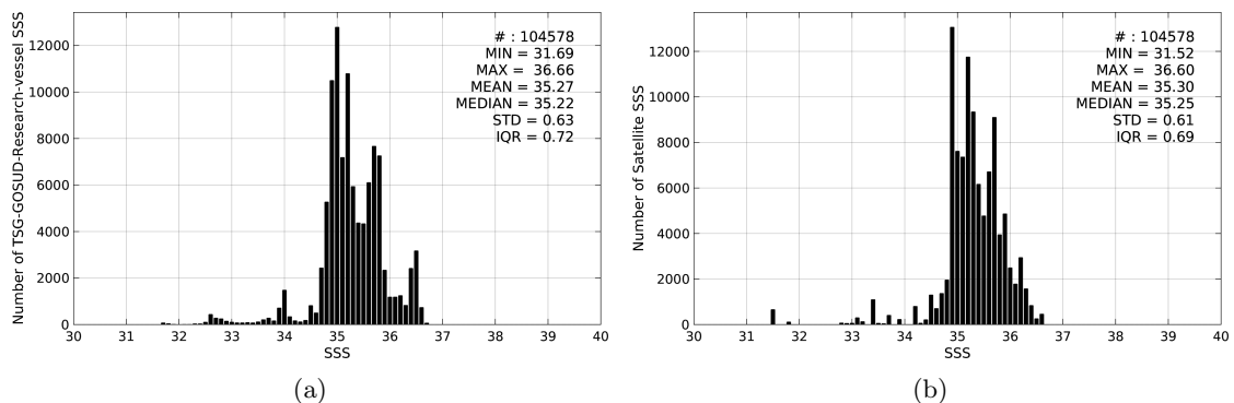
Figure 2: Histograms of SSS from TSG-GOSUD-Research-vessel (a) and Aquarius-L3-JPL-V4-7DAY-RUNNING (b) considering all match-up pairs per bins of 0.1 over the South Pacific Ocean Pi-MEP region and for the full satellite product period.
