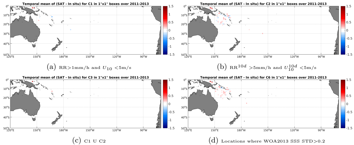
Figure 11: Temporal mean gridded over spatial boxes of size 1^\circ \times 1^\circ of \Delta SSS (Aquarius-L3-JPL-V4-7DAY-RUNNING - Surface drifters) for 4 different subdatasets corresponding to: RR > 1\text{mm/h} and U_{10} < 5\text{m/s} (a), RR^{10d} > 5\text{mm/h} and U_{10}^{10d} < 5\text{m/s} (b), C1 U C2 (c), Locations where WOA2013 SSS STD > 0.2 (d).
