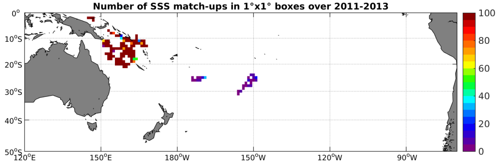
Figure 3: Number of SSS match-ups between Surface drifters SSS and the Aquarius-L3-JPL-V4-7DAY-RUNNING SSS product for the South Pacific Ocean Pi-MEP region over 1^\circ \times 1^\circ boxes and for the full satellite product period.
