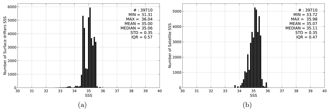
Figure 2: Histograms of SSS from Surface drifters (a) and Aquarius-L3-JPL-V4-7DAY-RUNNING (b) considering all match-up pairs per bins of 0.1 over the South Pacific Ocean Pi-MEP region and for the full satellite product period.
