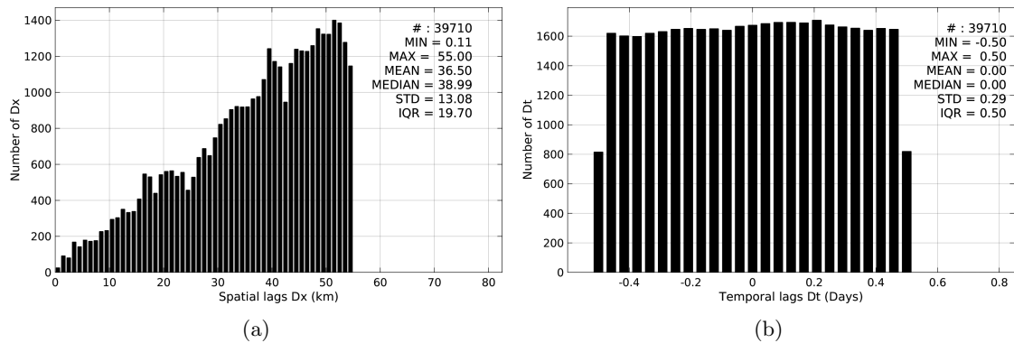
Figure 4: Histograms of the spatial (a) and temporal (b) lags between the time of the Surface drifters measurements and the date of the corresponding Aquarius-L3-JPL-V4-7DAY-RUNNING SSS product.
