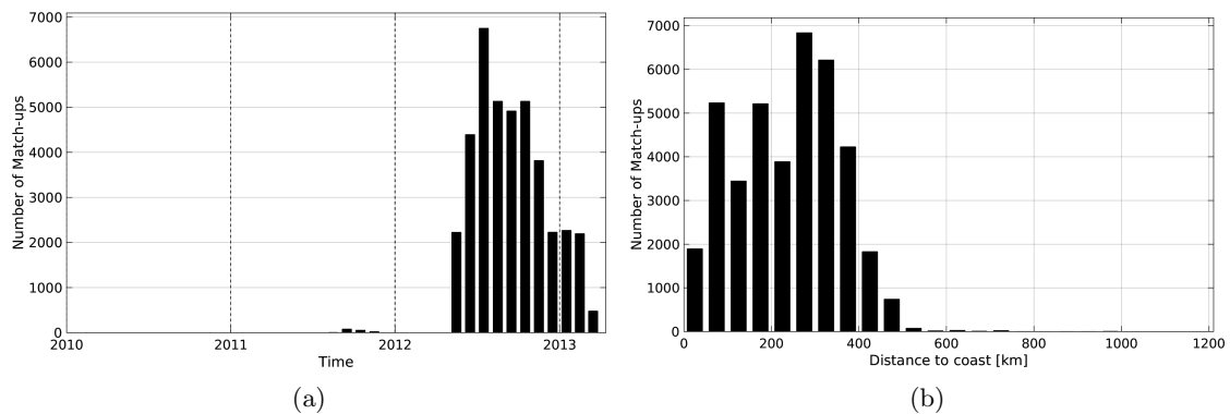
Figure 1: Number of match-ups between Surface drifters and Aquarius-L3-JPL-V4-7DAY-RUNNING SSS as a function of time (a) and as function of the distance to coast (b) over the South Pacific Ocean Pi-MEP region and for the full satellite product period.
