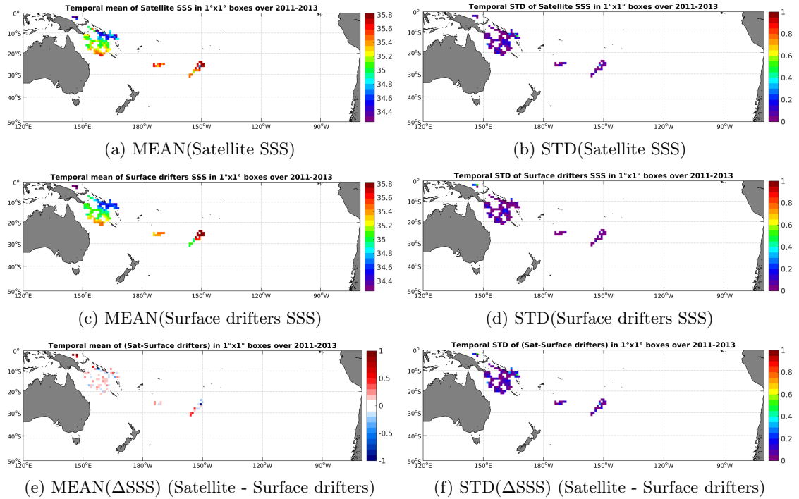
Figure 5: Temporal mean (left) and STD (right) of SSS from Aquarius-L3-JPL-V4-7DAY-RUNNING (top), Surface drifters (middle), and of \Delta SSS (Satellite - Surface drifters). Only match-up pairs are used to generate these maps.
