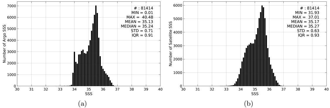
Figure 2: Histograms of SSS from Argo (a) and Aquarius-L3-JPL-V4-7DAY-RUNNING (b) considering all match-up pairs per bins of 0.1 over the South Pacific Ocean Pi-MEP region and for the full satellite product period.
