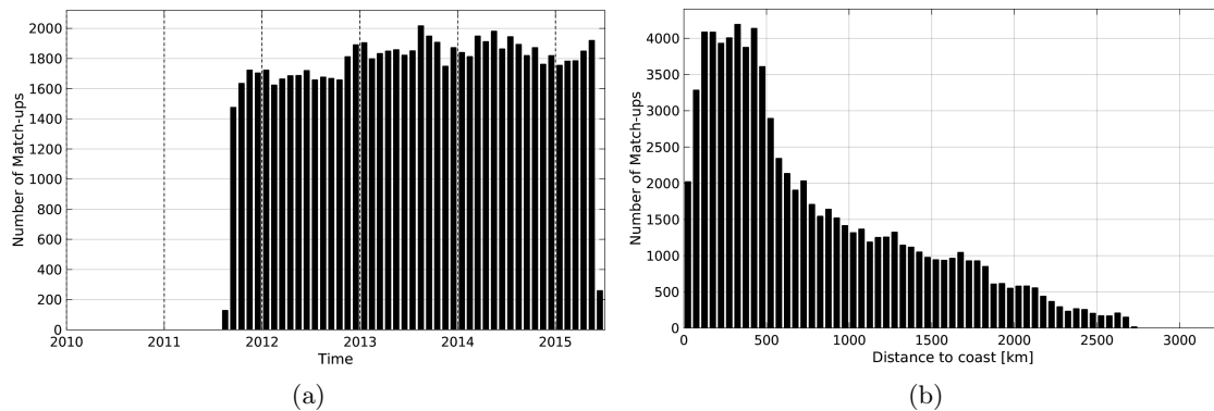
Figure 1: Number of match-ups between Argo and Aquarius-L3-JPL-V4-7DAY-RUNNING SSS as a function of time (a) and as function of the distance to coast (b) over the South Pacific Ocean Pi-MEP region and for the full satellite product period.
