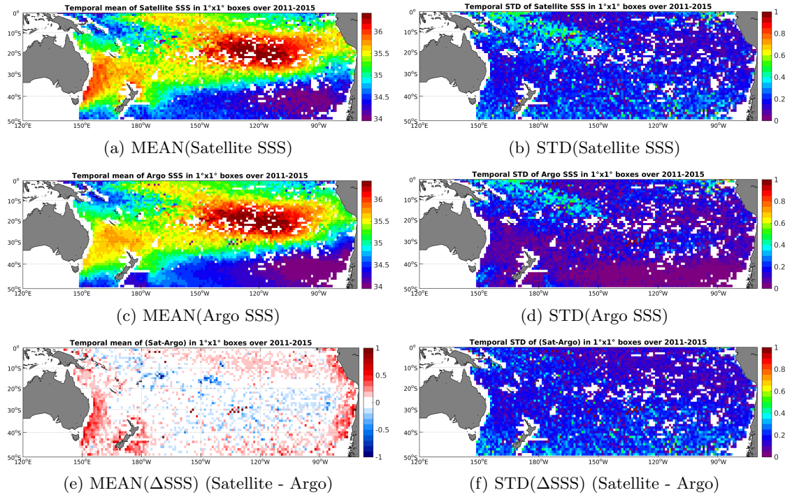
Figure 6: Temporal mean (left) and STD (right) of SSS from Aquarius-L3-JPL-V4-7DAY-RUNNING (top), Argo (middle), and of \Delta SSS (Satellite - Argo). Only match-up pairs are used to generate these maps.
