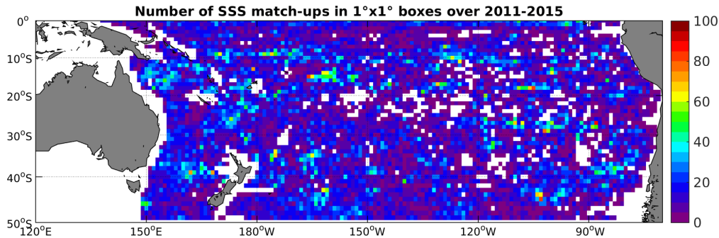
Figure 4: Number of SSS match-ups between Argo SSS and the Aquarius-L3-JPL-V4-7DAY-RUNNING SSS product for the South Pacific Ocean Pi-MEP region over 1^\circ \times 1^\circ boxes and for the full satellite product period.
