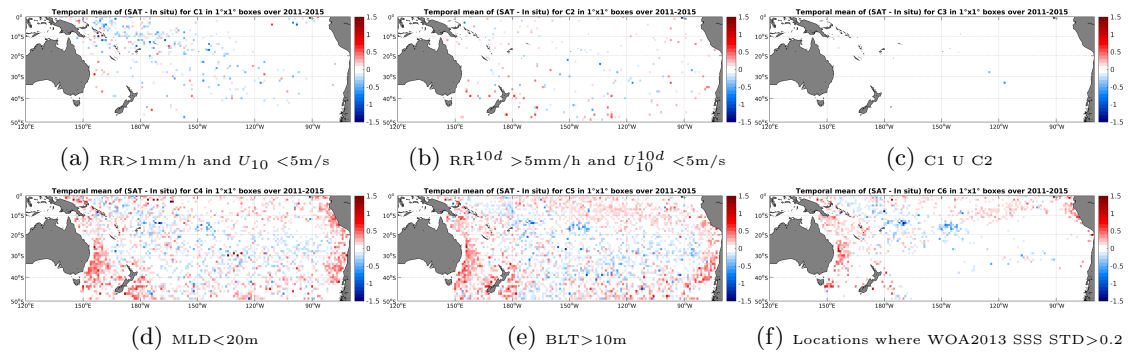
Figure 12: Temporal mean gridded over spatial boxes of size 1^\circ \times 1^\circ of \Delta SSS (Aquarius-L3-JPL-V4-7DAY-RUNNING - Argo) for 6 different subdatasets corresponding to:RR >1 mm/h and U_{10} < 5 m/s (a), RR^{10d} > 5 mm/h and U_{10}^{10d} < 5 m/s (b), C1 U C2 (c),MLD <20 m (d),BLT >10 m (e),Locations where WOA2013 SSS STD >0.2 (f).
