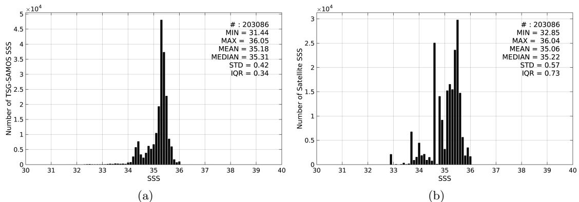
Figure 2: Histograms of SSS from TSG-SAMOS (a) and Aquarius-L3-JPL-V4-MONTHLY (b) considering all match-up pairs per bins of 0.1 over the South Pacific Ocean Pi-MEP region and for the full satellite product period.
