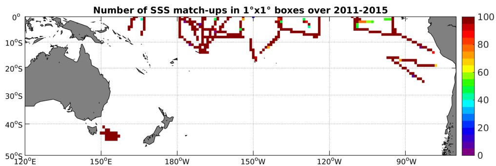
Figure 4: Number of SSS match-ups between TSG-SAMOS SSS and the Aquarius-L3-JPL-V4-MONTHLY SSS product for the South Pacific Ocean Pi-MEP region over 1^\circ \times 1^\circ boxes and for the full satellite product period.
