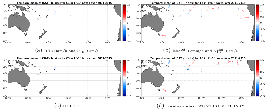
Figure 12: Temporal mean gridded over spatial boxes of size 1^\circ \times 1^\circ of \Delta SSS (Aquarius-L3-JPL-V4-MONTHLY - TSG-SAMOS) for 4 different subdatasets corresponding to: RR > 1\text{mm/h} and U_{10} < 5\text{m/s} (a), RR^{10d} > 5\text{mm/h} and U_{10}^{10d} < 5\text{m/s} (b), C1 U C2 (c), Locations where WOA2013 SSS STD > 0.2 (d).
