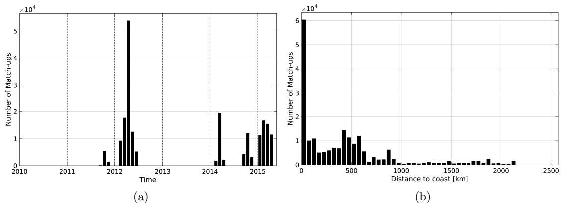
Figure 1: Number of match-ups between TSG-SAMOS and Aquarius-L3-JPL-V4-MONTHLY SSS as a function of time (a) and as function of the distance to coast (b) over the South Pacific Ocean Pi-MEP region and for the full satellite product period.
