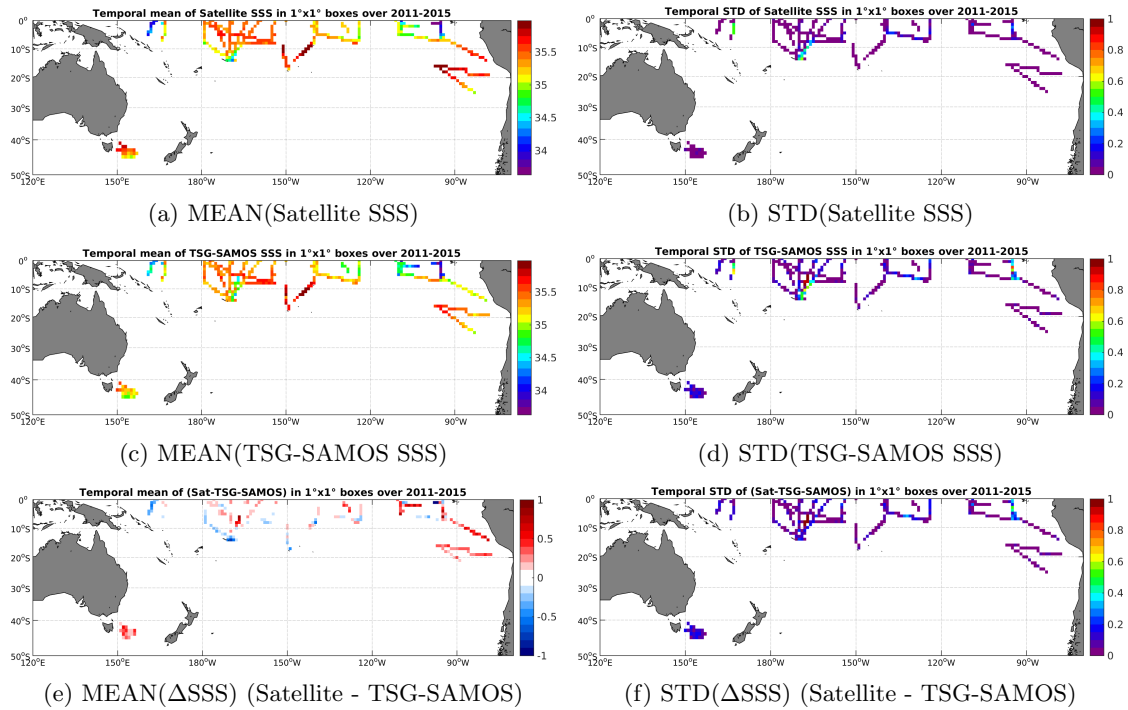
Figure 6: Temporal mean (left) and STD (right) of SSS from Aquarius-L3-JPL-V4-MONTHLY (top), TSG-SAMOS (middle), and of \Delta SSS (Satellite - TSG-SAMOS). Only match-up pairs are used to generate these maps.
