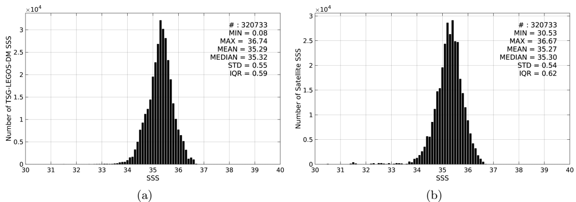
Figure 2: Histograms of SSS from TSG-LEGOS-DM (a) and Aquarius-L3-JPL-V4-MONTHLY (b) considering all match-up pairs per bins of 0.1 over the South Pacific Ocean Pi-MEP region and for the full satellite product period.
