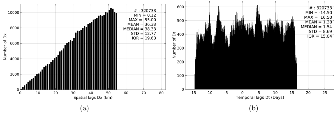
Figure 5: Histograms of the spatial (a) and temporal (b) lags between the time of the TSG-LEGOS-DM measurements and the date of the corresponding Aquarius-L3-JPL-V4-MONTHLY SSS product.
