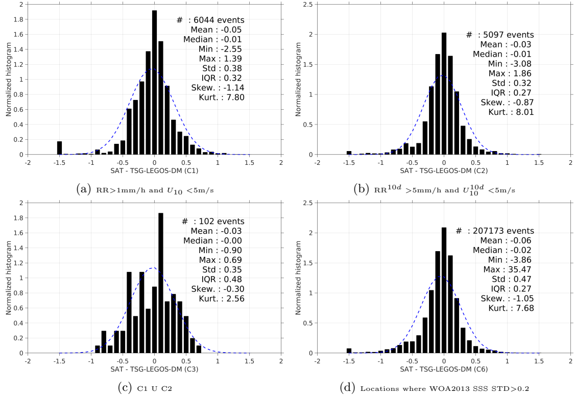
Figure 13: Normalized histogram of \Delta\text{SSS} (Aquarius-L3-JPL-V4-MONTHLY - TSG-LEGOS-DM) for 6 different subdatasets corresponding to: \text{RR} > 1\text{mm/h} and U_{10} < 5\text{m/s} (a), \text{RR}^{10d} > 5\text{mm/h} and U_{10}^{10d} < 5\text{m/s} (b), C1 U C2 (c), Locations where WOA2013 SSS STD > 0.2 (d).
