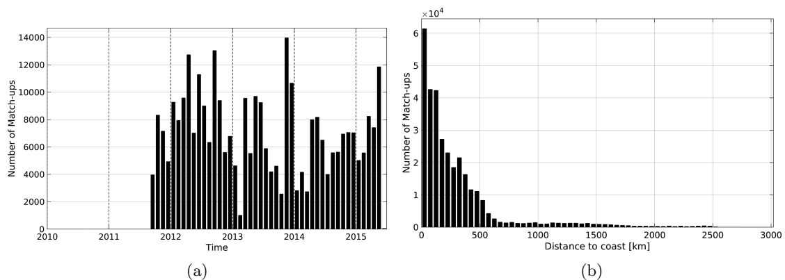
Figure 1: Number of match-ups between TSG-LEGOS-DM and Aquarius-L3-JPL-V4-MONTHLY SSS as a function of time (a) and as function of the distance to coast (b) over the South Pacific Ocean Pi-MEP region and for the full satellite product period.
