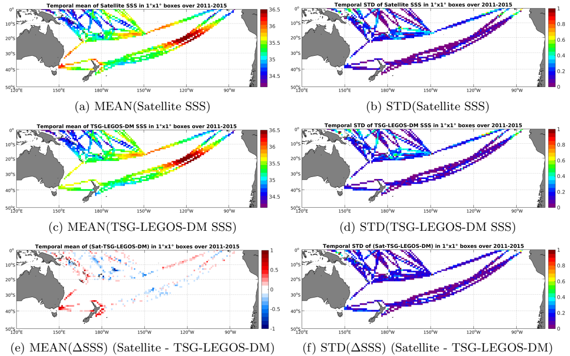
Figure 6: Temporal mean (left) and STD (right) of SSS from Aquarius-L3-JPL-V4-MONTHLY (top), TSG-LEGOS-DM (middle), and of \Delta SSS (Satellite - TSG-LEGOS-DM). Only match-up pairs are used to generate these maps.
