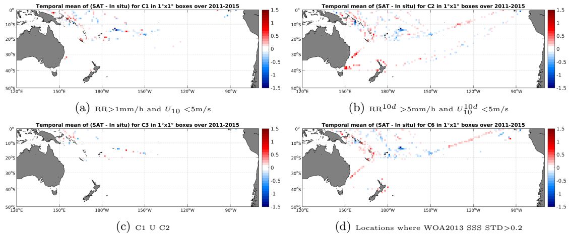
Figure 12: Temporal mean gridded over spatial boxes of size 1^\circ \times 1^\circ of \Delta SSS (Aquarius-L3-JPL-V4-MONTHLY - TSG-LEGOS-DM) for 4 different subdatasets corresponding to:RR>1mm/h and U_{10} < 5\text{m/s} (a), RR^{10d} > 5\text{mm/h} and U_{10}^{10d} < 5\text{m/s} (b), C1 U C2 (c),Locations where WOA2013 SSS STD>0.2 (d).
