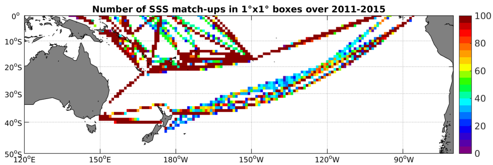
Figure 4: Number of SSS match-ups between TSG-LEGOS-DM SSS and the Aquarius-L3-JPL-V4-MONTHLY SSS product for the South Pacific Ocean Pi-MEP region over 1^\circ \times 1^\circ boxes and for the full satellite product period.
