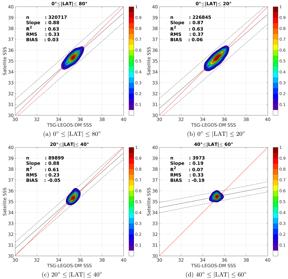
Figure 9: Contour maps of the concentration of Aquarius-L3-JPL-V4-MONTHLY SSS (y-axis) versus TSG-LEGOS-DM SSS (x-axis) at match-up pairs for different latitude bands. For each plot, the red line shows x=y . The black thin and dashed lines indicate a linear fit through the data cloud and the \pm 95\% confidence levels, respectively. The number match-up pairs n , the slope and R^2 coefficient of the linear fit, the root mean square (RMS) and the mean bias between satellite and in situ data are indicated for each latitude band in each plots.
