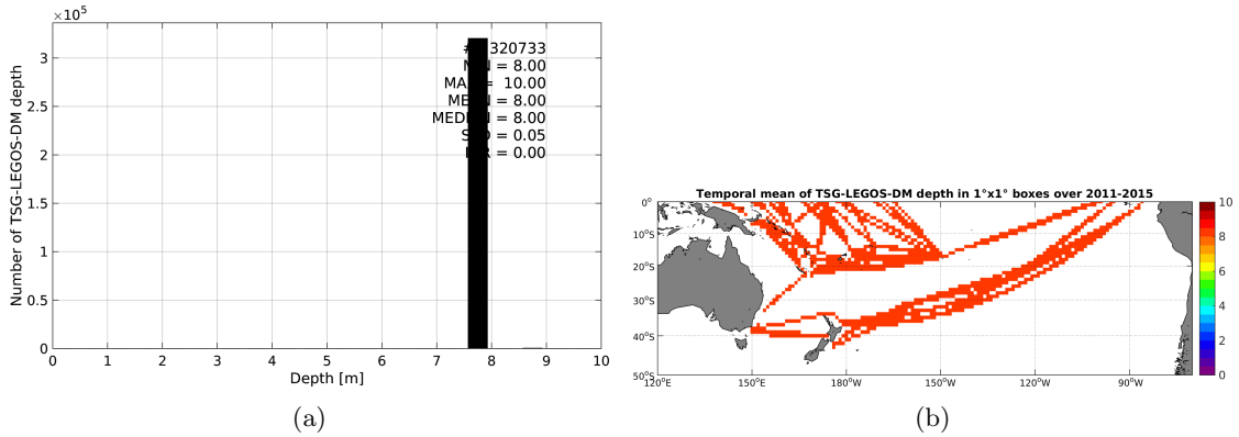
Figure 3: Histograms of the depth of the upper level SSS measurements from TSG-LEGOS-DM in the Match-up DataBase for the South Pacific Ocean Pi-MEP region (a) and temporal mean spatial distribution of pressure of the in situ SSS data over 1^\circ \times 1^\circ boxes and for the full satellite product period (b).
