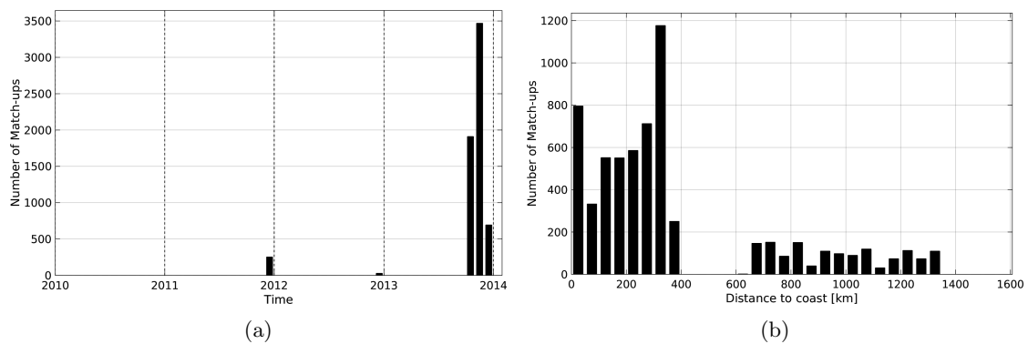
Figure 1: Number of match-ups between TSG-GOSUD-Sailing-ship and Aquarius-L3-JPL-V4-MONTHLY SSS as a function of time (a) and as function of the distance to coast (b) over the South Pacific Ocean Pi-MEP region and for the full satellite product period.
