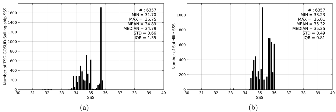
Figure 2: Histograms of SSS from TSG-GOSUD-Sailing-ship (a) and Aquarius-L3-JPL-V4-MONTHLY (b) considering all match-up pairs per bins of 0.1 over the South Pacific Ocean Pi-MEP region and for the full satellite product period.
