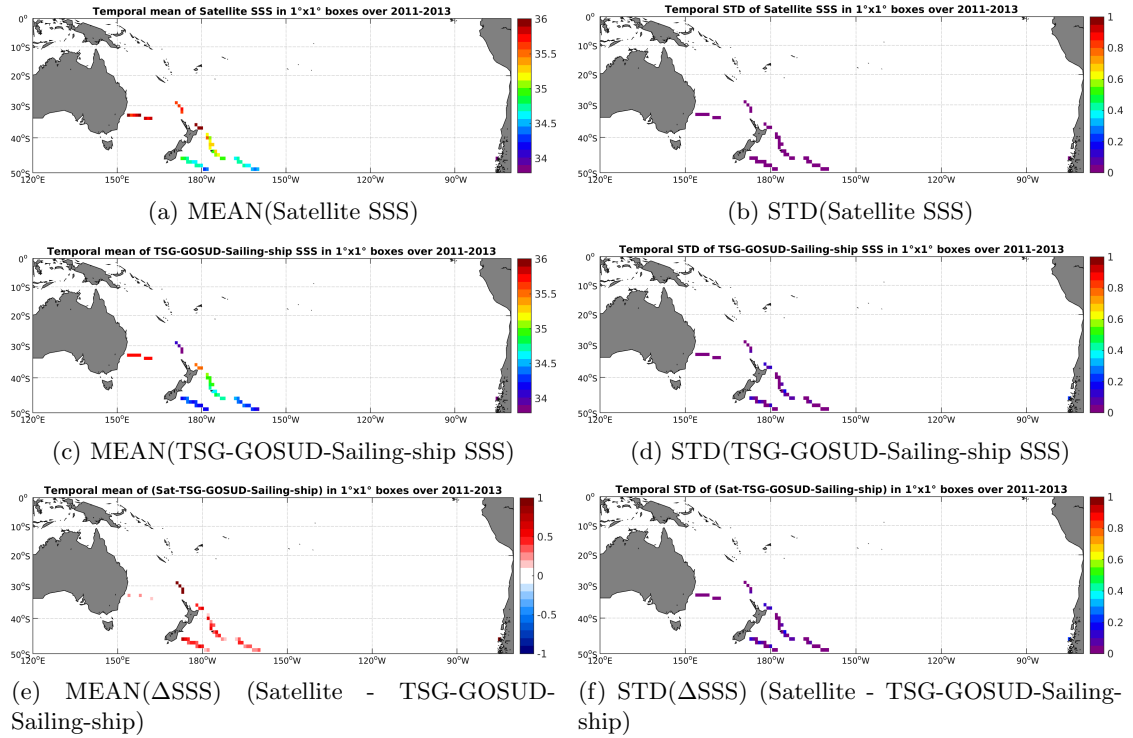
Figure 6: Temporal mean (left) and STD (right) of SSS from Aquarius-L3-JPL-V4-MONTHLY (top), TSG-GOSUD-Sailing-ship (middle), and of \Delta SSS (Satellite - TSG-GOSUD-Sailing-ship). Only match-up pairs are used to generate these maps.
