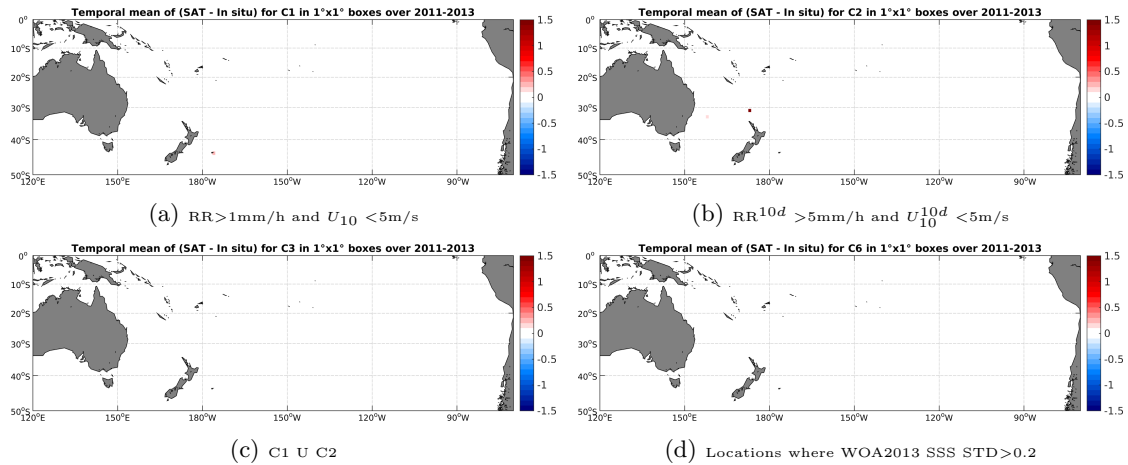
Figure 12: Temporal mean gridded over spatial boxes of size 1^\circ \times 1^\circ of \Delta SSS (Aquarius-L3-JPL-V4-MONTHLY - TSG-GOSUD-Sailing-ship) for 4 different subdatasets corresponding to: RR > 1\text{mm/h} and U_{10} < 5\text{m/s} (a), RR^{10d} > 5\text{mm/h} and U_{10}^{10d} < 5\text{m/s} (b), C1 U C2 (c), Locations where WOA2013 SSS STD > 0.2 (d).
