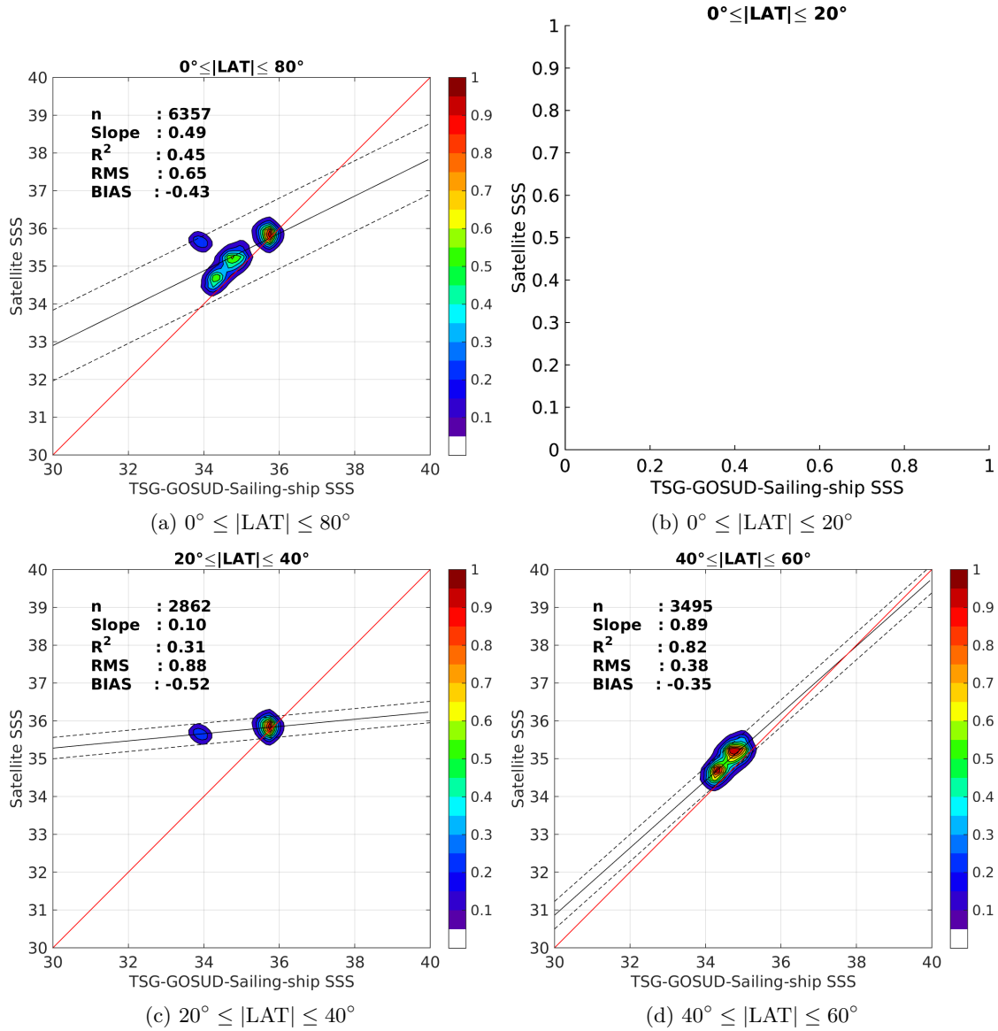
Figure 9: Contour maps of the concentration of Aquarius-L3-JPL-V4-MONTHLY SSS (y-axis) versus TSG-GOSUD-Sailing-ship SSS (x-axis) at match-up pairs for different latitude bands. For each plot, the red line shows x=y . The black thin and dashed lines indicate a linear fit through the data cloud and the \pm 95\% confidence levels, respectively. The number match-up pairs n , the slope and R^2 coefficient of the linear fit, the root mean square (RMS) and the mean bias between satellite and in situ data are indicated for each latitude band in each plots.
