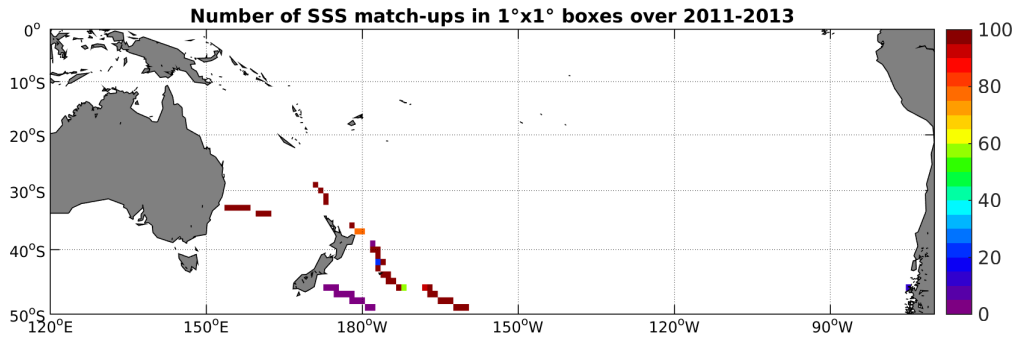
Figure 4: Number of SSS match-ups between TSG-GOSUD-Sailing-ship SSS and the Aquarius-L3-JPL-V4-MONTHLY SSS product for the South Pacific Ocean Pi-MEP region over 1^\circ \times 1^\circ boxes and for the full satellite product period.
