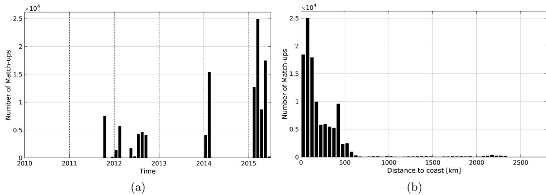
Figure 1: Number of match-ups between TSG-GOSUD-Research-vessel and Aquarius-L3-JPL-V4-MONTHLY SSS as a function of time (a) and as function of the distance to coast (b) over the South Pacific Ocean Pi-MEP region and for the full satellite product period.
