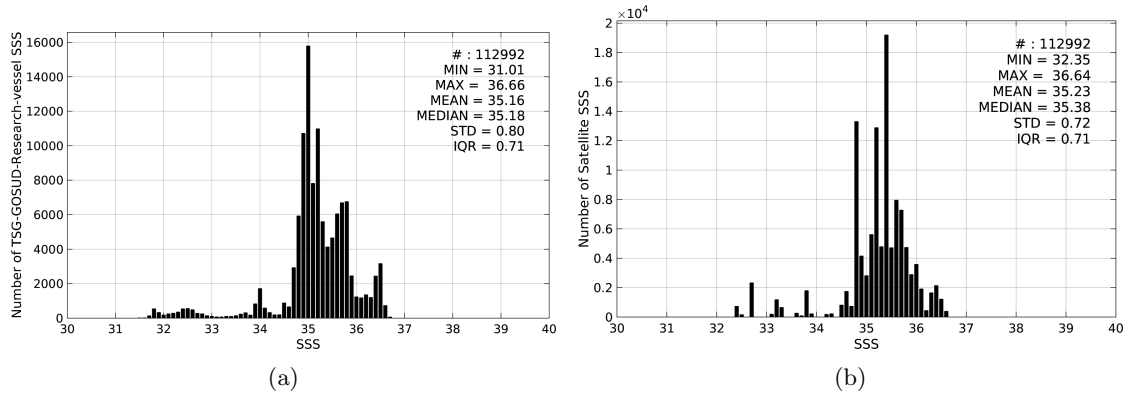
Figure 2: Histograms of SSS from TSG-GOSUD-Research-vessel (a) and Aquarius-L3-JPL-V4-MONTHLY (b) considering all match-up pairs per bins of 0.1 over the South Pacific Ocean Pi-MEP region and for the full satellite product period.
