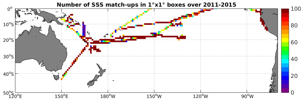
Figure 4: Number of SSS match-ups between TSG-GOSUD-Research-vessel SSS and the Aquarius-L3-JPL-V4-MONTHLY SSS product for the South Pacific Ocean Pi-MEP region over 1^\circ \times 1^\circ boxes and for the full satellite product period.
