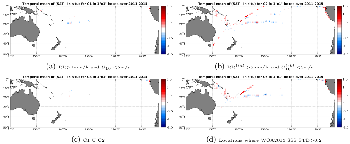
Figure 12: Temporal mean gridded over spatial boxes of size 1^\circ \times 1^\circ of \Delta SSS (Aquarius-L3-JPL-V4-MONTHLY - TSG-GOSUD-Research-vessel) for 4 different subdatasets corresponding to: RR > 1\text{mm/h} and U_{10} < 5\text{m/s} (a), RR^{10d} > 5\text{mm/h} and U_{10}^{10d} < 5\text{m/s} (b), C1 U C2 (c), Locations where WOA2013 SSS STD > 0.2 (d).
