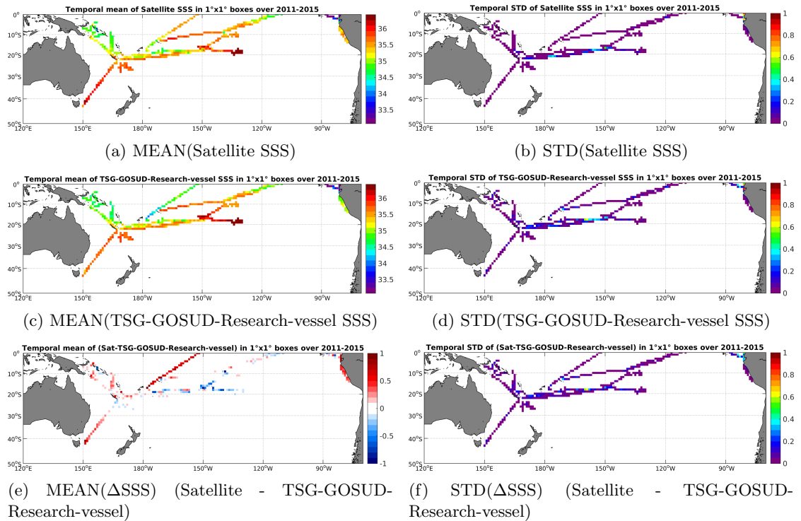
Figure 6: Temporal mean (left) and STD (right) of SSS from Aquarius-L3-JPL-V4-MONTHLY (top), TSG-GOSUD-Research-vessel (middle), and of \Delta SSS (Satellite - TSG-GOSUD-Research-vessel). Only match-up pairs are used to generate these maps.
