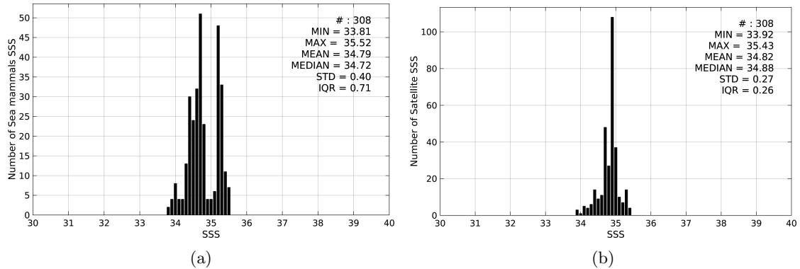
Figure 2: Histograms of SSS from Sea mammals (a) and Aquarius-L3-JPL-V4-MONTHLY (b) considering all match-up pairs per bins of 0.1 over the South Pacific Ocean Pi-MEP region and for the full satellite product period.
