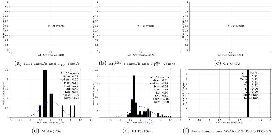
Figure 13: Normalized histogram of \Delta\text{SSS} (Aquarius-L3-JPL-V4-MONTHLY - Sea mammals) for 6 different subdatasets corresponding to: RR > 1\text{mm/h} and U_{10} < 5\text{m/s} (a), RR^{10d} > 5\text{mm/h} and U_{10}^{10d} < 5\text{m/s} (b), C1 U C2 (c), MLD < 20\text{m} (d), BLT > 10\text{m} (e), Locations where WOA2013 SSS STD > 0.2 (f).
