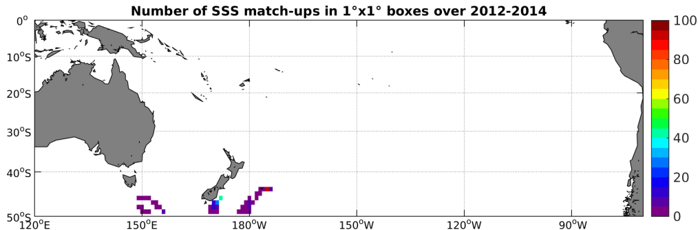
Figure 4: Number of SSS match-ups between Sea mammals SSS and the Aquarius-L3-JPL-V4-MONTHLY SSS product for the South Pacific Ocean Pi-MEP region over 1^\circ \times 1^\circ boxes and for the full satellite product period.
