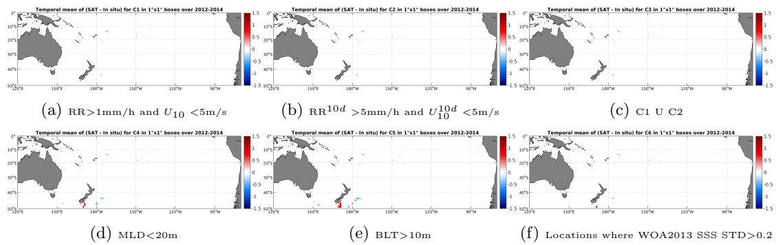
Figure 12: Temporal mean gridded over spatial boxes of size 1^\circ \times 1^\circ of \Delta SSS (Aquarius-L3-JPL-V4-MONTHLY - Sea mammals) for 6 different subdatasets corresponding to:RR >1 mm/h and U_{10} < 5 m/s (a), RR^{10d} > 5 mm/h and U_{10}^{10d} < 5 m/s (b), C1 U C2 (c),MLD <20 m (d),BLT >10 m (e),Locations where WOA2013 SSS STD >0.2 (f).
