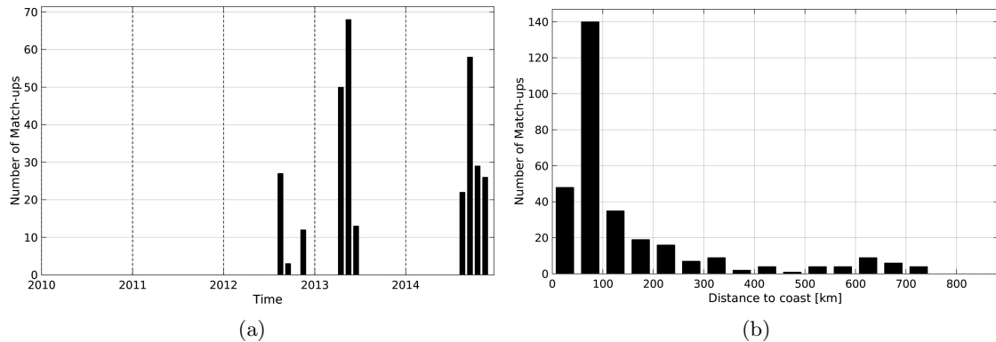
Figure 1: Number of match-ups between Sea mammals and Aquarius-L3-JPL-V4-MONTHLY SSS as a function of time (a) and as function of the distance to coast (b) over the South Pacific Ocean Pi-MEP region and for the full satellite product period.
