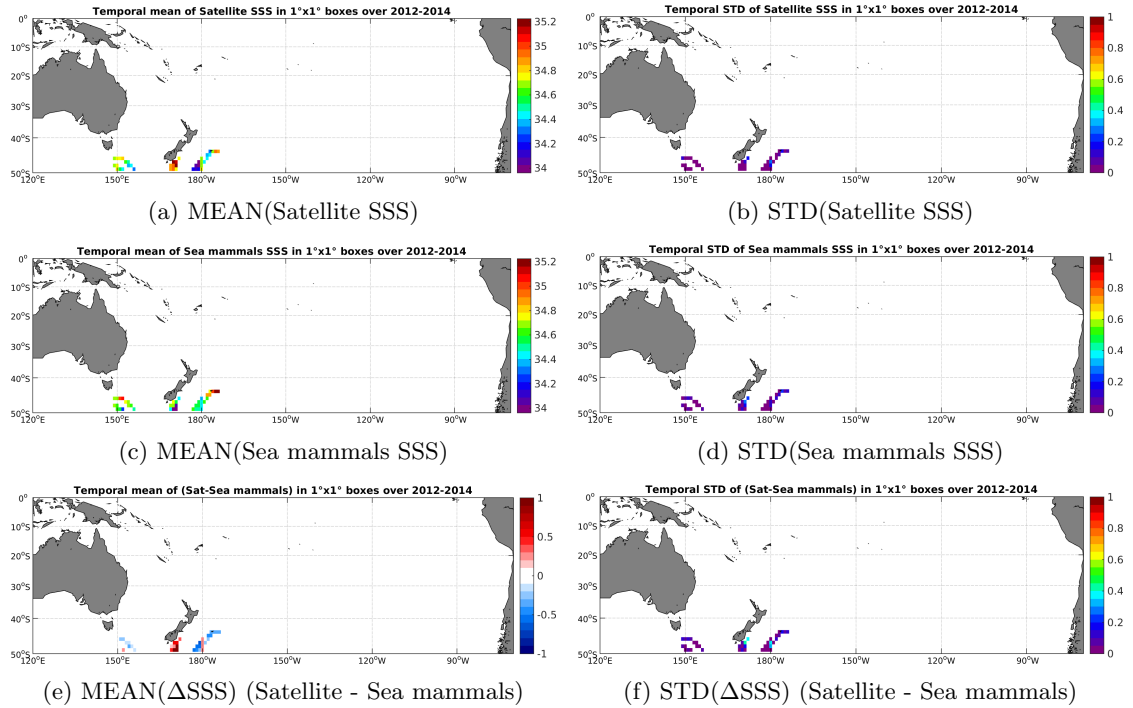
Figure 6: Temporal mean (left) and STD (right) of SSS from Aquarius-L3-JPL-V4-MONTHLY (top), Sea mammals (middle), and of \Delta SSS (Satellite - Sea mammals). Only match-up pairs are used to generate these maps.
