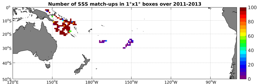
Figure 3: Number of SSS match-ups between Surface drifters SSS and the Aquarius-L3-JPL-V4-MONTHLY SSS product for the South Pacific Ocean Pi-MEP region over 1^\circ \times 1^\circ boxes and for the full satellite product period.
