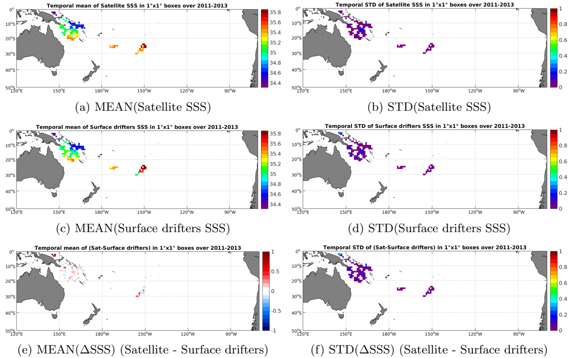
Figure 5: Temporal mean (left) and STD (right) of SSS from Aquarius-L3-JPL-V4-MONTHLY (top), Surface drifters (middle), and of \Delta SSS (Satellite - Surface drifters). Only match-up pairs are used to generate these maps.
