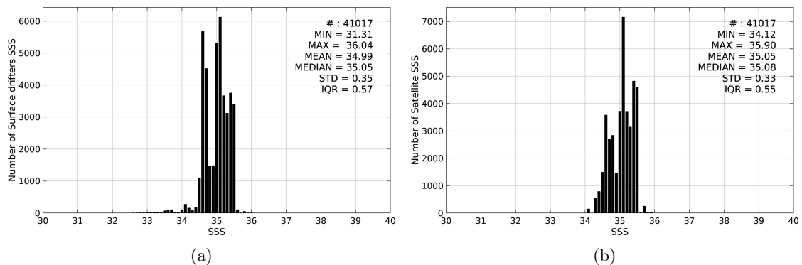
Figure 2: Histograms of SSS from Surface drifters (a) and Aquarius-L3-JPL-V4-MONTHLY (b) considering all match-up pairs per bins of 0.1 over the South Pacific Ocean Pi-MEP region and for the full satellite product period.
