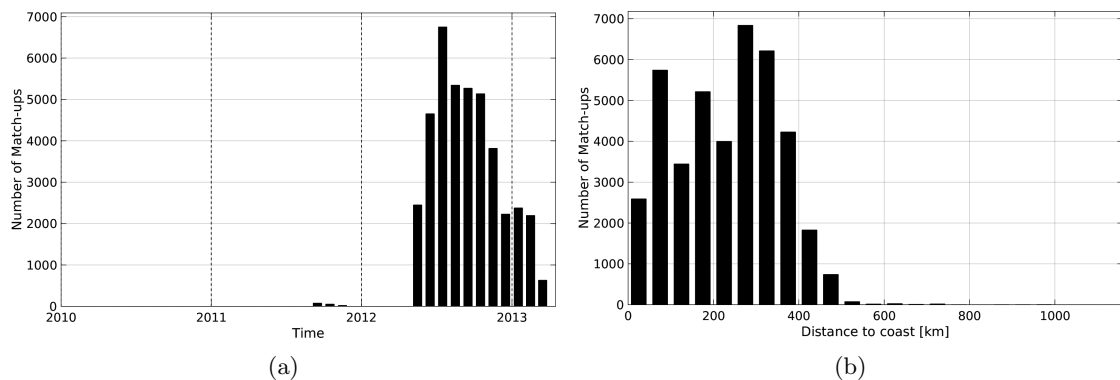
Figure 1: Number of match-ups between Surface drifters and Aquarius-L3-JPL-V4-MONTHLY SSS as a function of time (a) and as function of the distance to coast (b) over the South Pacific Ocean Pi-MEP region and for the full satellite product period.
