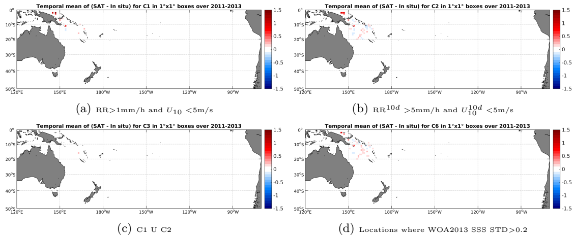
Figure 11: Temporal mean gridded over spatial boxes of size 1^\circ \times 1^\circ of \Delta SSS (Aquarius-L3-JPL-V4-MONTHLY - Surface drifters) for 4 different subdatasets corresponding to: RR > 1\text{mm/h} and U_{10} < 5\text{m/s} (a), RR^{10d} > 5\text{mm/h} and U_{10}^{10d} < 5\text{m/s} (b), C1 U C2 (c), Locations where WOA2013 SSS STD > 0.2 (d).
