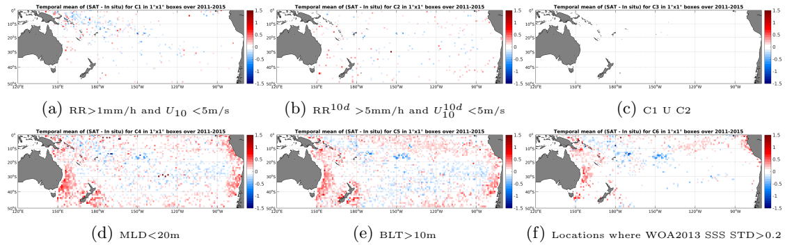
Figure 12: Temporal mean gridded over spatial boxes of size 1^\circ \times 1^\circ of \Delta SSS (Aquarius-L3-JPL-V4-MONTHLY - Argo) for 6 different subdatasets corresponding to:RR >1 mm/h and U_{10} < 5 m/s (a), RR^{10d} > 5 mm/h and U_{10}^{10d} < 5 m/s (b), C1 U C2 (c),MLD <20 m (d),BLT >10 m (e),Locations where WOA2013 SSS STD >0.2 (f).
