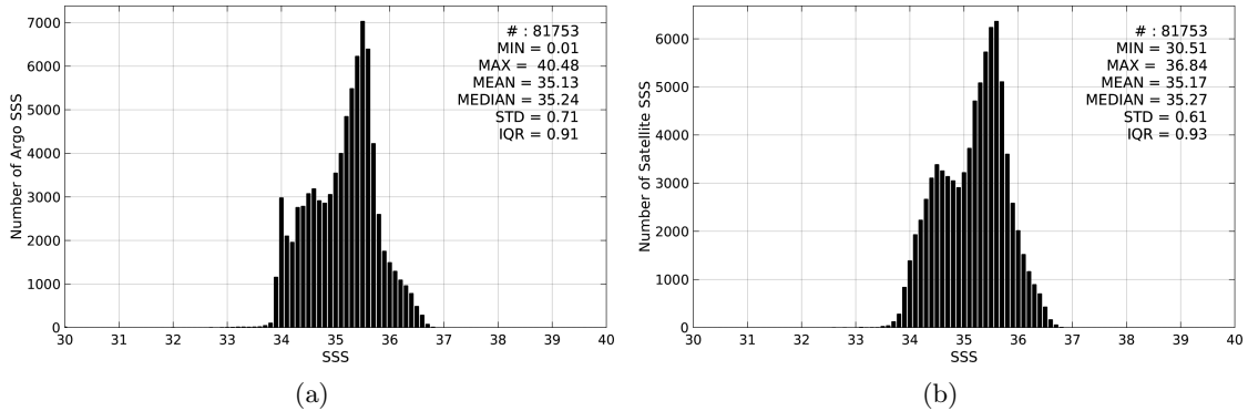
Figure 2: Histograms of SSS from Argo (a) and Aquarius-L3-JPL-V4-MONTHLY (b) considering all match-up pairs per bins of 0.1 over the South Pacific Ocean Pi-MEP region and for the full satellite product period.
