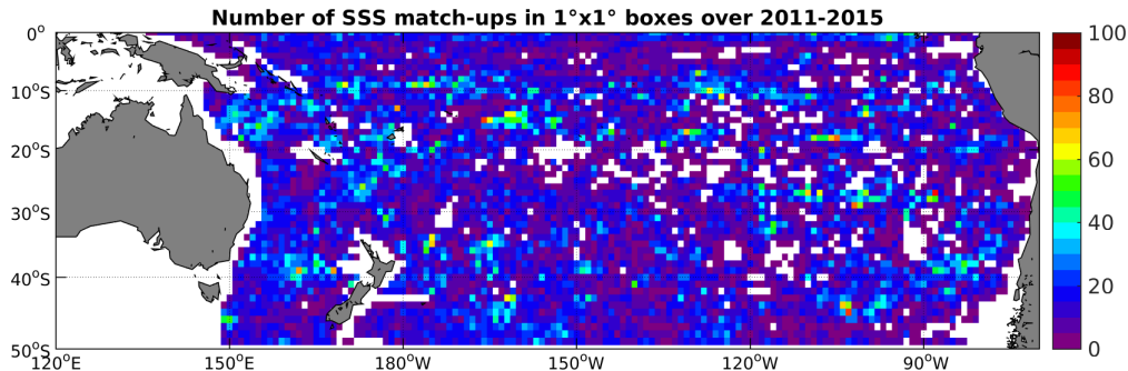
Figure 4: Number of SSS match-ups between Argo SSS and the Aquarius-L3-JPL-V4-MONTHLY SSS product for the South Pacific Ocean Pi-MEP region over 1^\circ \times 1^\circ boxes and for the full satellite product period.
