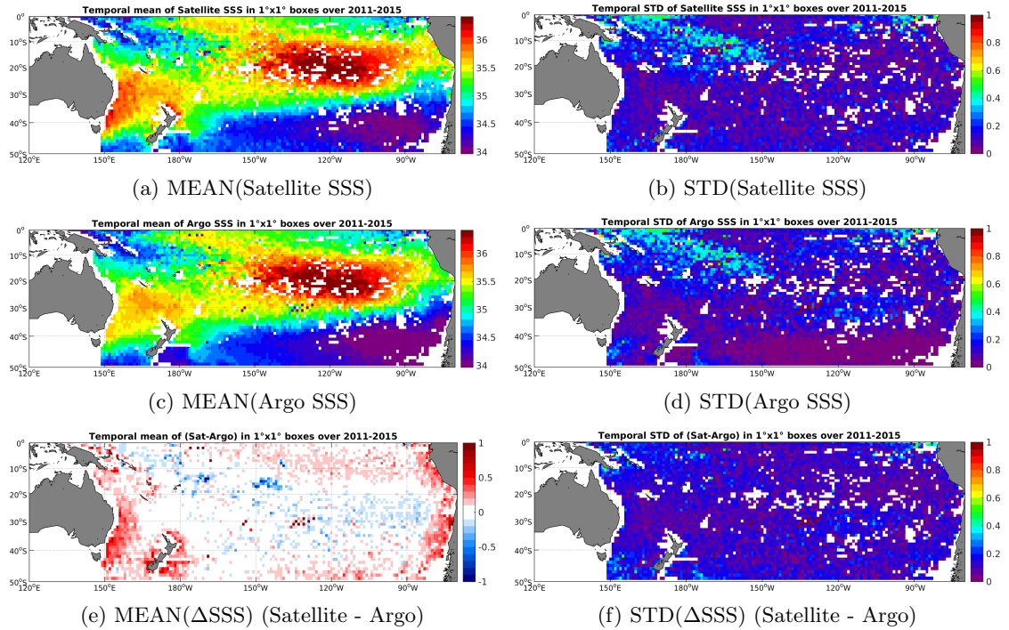
Figure 6: Temporal mean (left) and STD (right) of SSS from Aquarius-L3-JPL-V4-MONTHLY (top), Argo (middle), and of \Delta SSS (Satellite - Argo). Only match-up pairs are used to generate these maps.
