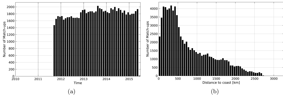
Figure 1: Number of match-ups between Argo and Aquarius-L3-JPL-V4-MONTHLY SSS as a function of time (a) and as function of the distance to coast (b) over the South Pacific Ocean Pi-MEP region and for the full satellite product period.
