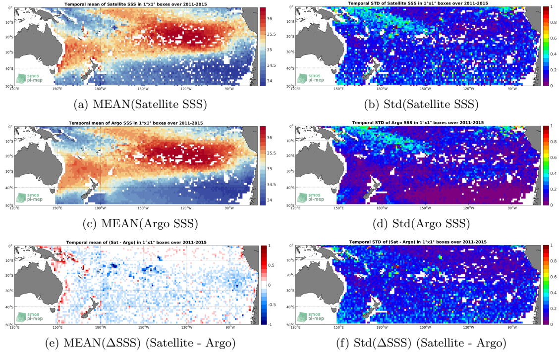
Figure 6: Temporal mean (left) and Std (right) of SSS from Aquarius SSS L2-AVERAGED OR v5 (NASA-GSFC) (top), Argo (middle), and of \Delta SSS (Satellite - Argo). Only match-up pairs are used to generate these maps.
