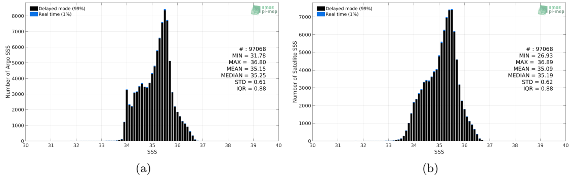
Figure 2: Histograms of SSS from Argo (a) and Aquarius SSS L2-AVERAGED OR v5 (NASA-GSFC) (b) considering all match-up pairs per bins of 0.1 over the South Pacific Ocean Pi-MEP region and for the full satellite product period.
