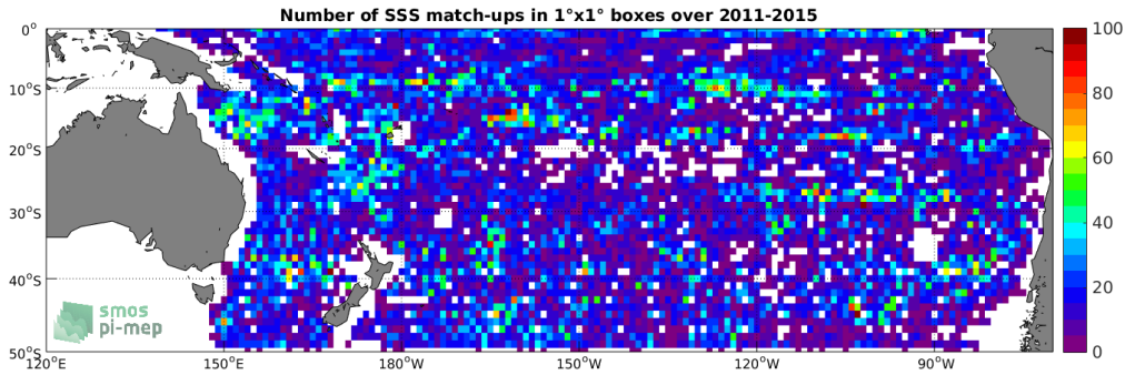
Figure 4: Number of SSS match-ups between Argo SSS and the Aquarius SSS L2-AVERAGED OR v5 (NASA-GSFC) SSS product for the South Pacific Ocean Pi-MEP region over 1^\circ \times 1^\circ boxes and for the full satellite product period.
