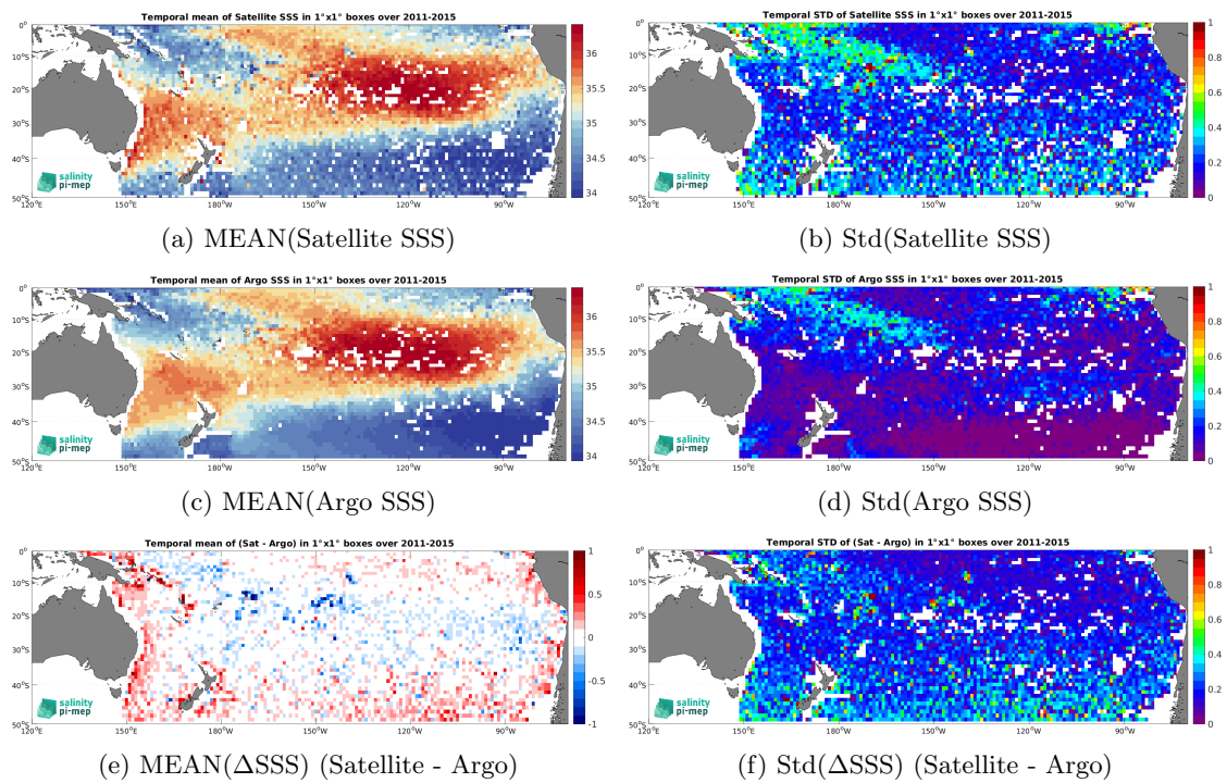
Figure 5: Temporal mean (left) and Std (right) of SSS from Aquarius SSS L2-AVERAGED CAP v5 (JPL) (top), Argo (middle), and of \Delta SSS (Satellite - Argo). Only match-up pairs are used to generate these maps.
