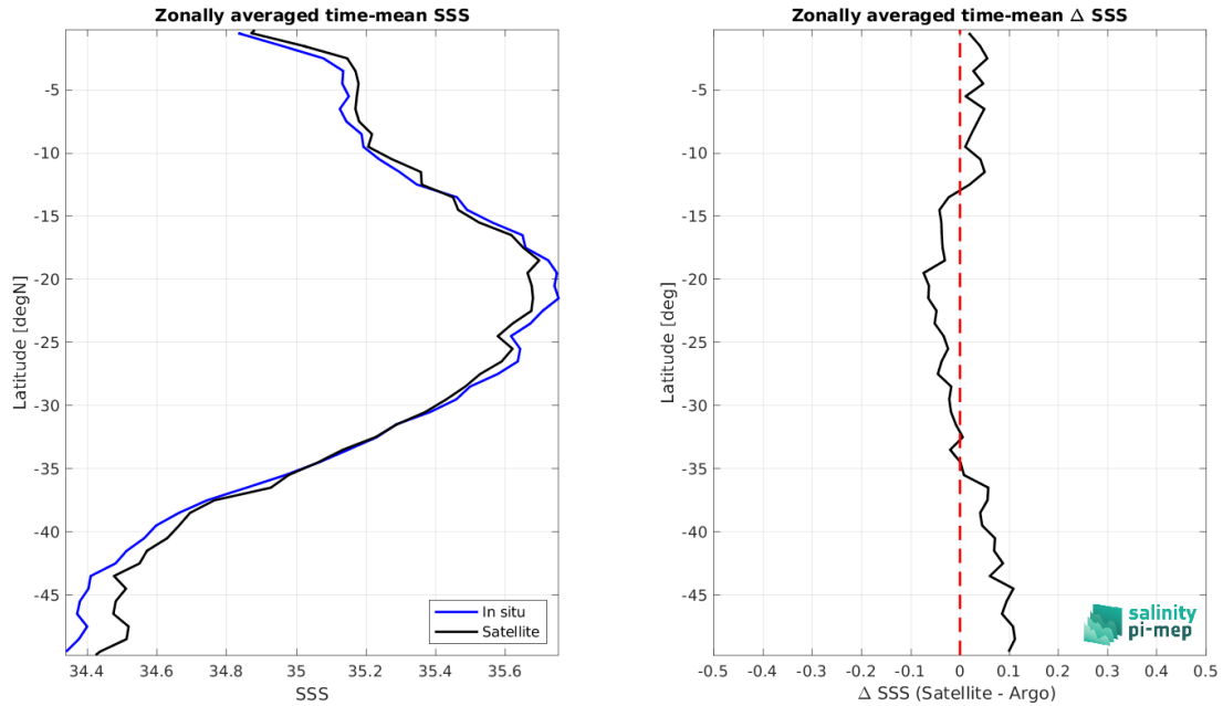
Figure 7: Left panel: Zonal mean SSS from Aquarius SSS L2-AVERAGED CAP v5 (JPL) satellite product (black) and from Argo (blue). Right panel: Zonal mean of \Delta SSS (Satellite - Argo) for all the collected Pi-MEP match-up pairs estimated over the full satellite product period.
