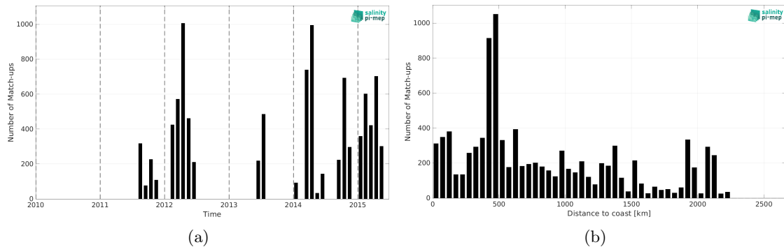
Figure 2: Number of match-ups between TSG (SAMOS) and Aquarius SSS L2 OR v5 (NASA-GSFC) SSS as a function of time (a) and as function of the distance to coast (b) over the South Pacific Ocean Pi-MEP region and for the full satellite product period.
