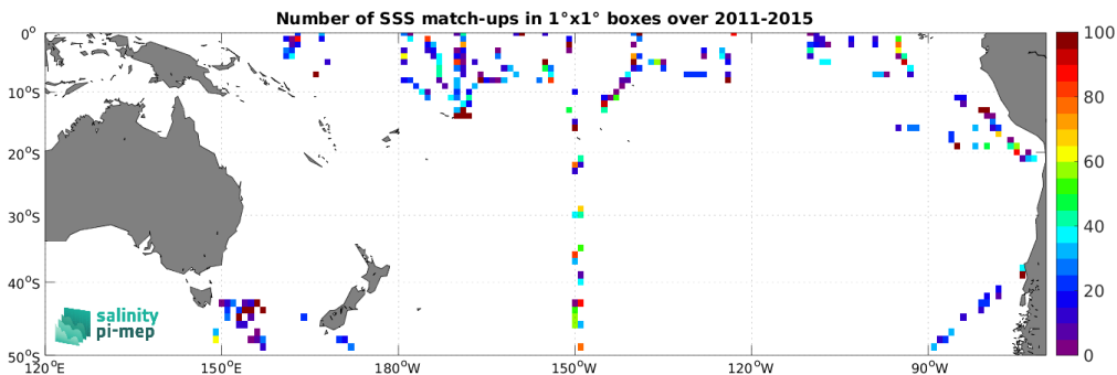
Figure 5: Number of SSS match-ups between TSG (SAMOS) SSS and the Aquarius SSS L2 OR v5 (NASA-GSFC) SSS product for the South Pacific Ocean Pi-MEP region over 1^\circ \times 1^\circ boxes and for the full satellite product period.
