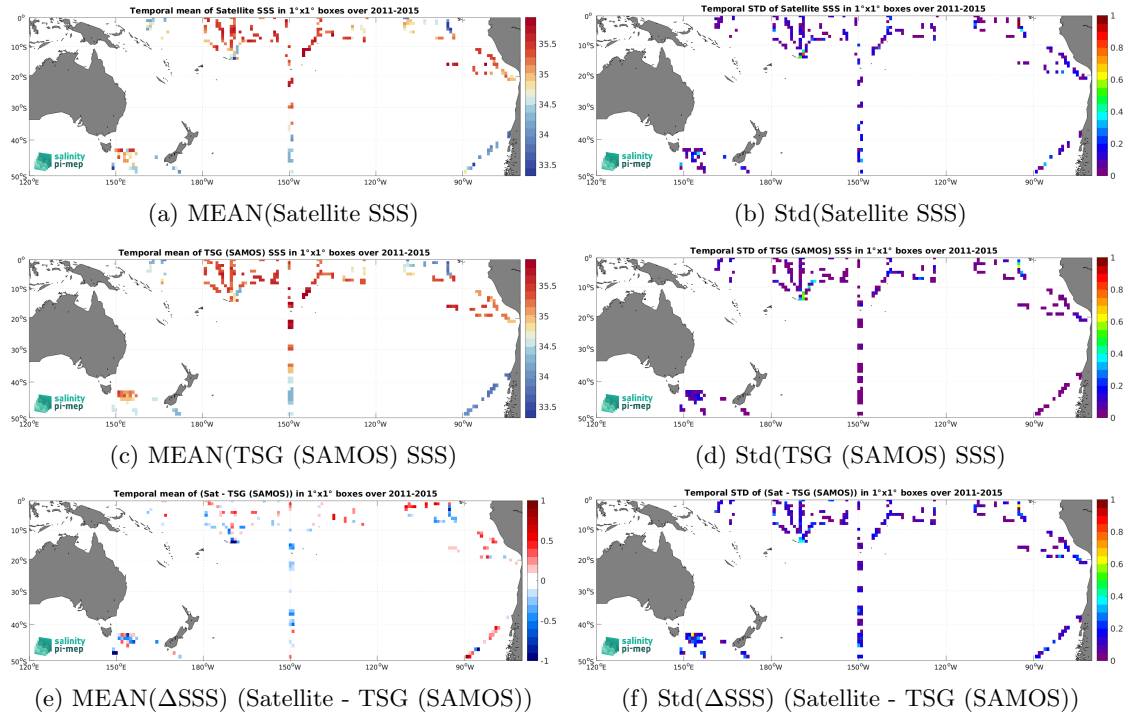
Figure 7: Temporal mean (left) and Std (right) of SSS from Aquarius SSS L2 OR v5 (NASA-GSFC) (top), TSG (SAMOS) (middle), and of \Delta SSS (Satellite - TSG (SAMOS)). Only match-up pairs are used to generate these maps.
