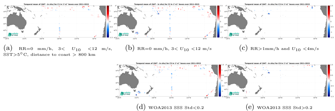
Figure 14: Temporal mean gridded over spatial boxes of size 1^\circ \times 1^\circ of \Delta SSS (Aquarius SSS L2 OR v5 (NASA-GSFC) - TSG (SAMOS)) for 5 different subdatasets corresponding to:RR=0 mm/h, 3 < U_{10} < 12 m/s, SST >5^\circ\text{C} , distance to coast > 800 km (a), RR=0 mm/h, 3 < U_{10} < 12 m/s (b), RR >1 mm/h and U_{10} < 4 m/s (c), WOA2013 SSS Std <0.2 (d), WOA2013 SSS Std >0.2 (e).
