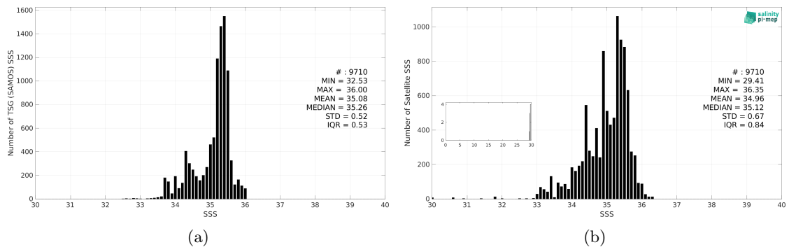
Figure 3: Histograms of SSS from TSG (SAMOS) (a) and Aquarius SSS L2 OR v5 (NASA-GSFC) (b) considering all match-up pairs per bins of 0.1 over the South Pacific Ocean Pi-MEP region and for the full satellite product period.
