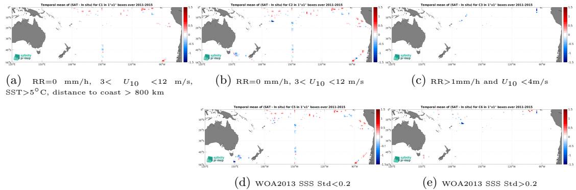
Figure 12: Temporal mean gridded over spatial boxes of size 1^\circ \times 1^\circ of \Delta\text{SSS} (Aquarius SSS L2 OR v5 (NASA-GSFC) - TSG (SAMOS)) for 5 different subdatasets corresponding to:RR=0 mm/h, 3 < U_{10} < 12 m/s, SST >5^\circ\text{C} , distance to coast > 800 km (a), RR=0 mm/h, 3 < U_{10} < 12 m/s (b), RR >1 mm/h and U_{10} < 4 m/s (c), WOA2013 SSS Std <0.2 (d), WOA2013 SSS Std >0.2 (e).
