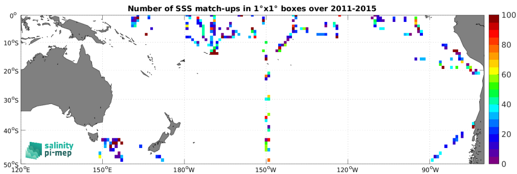
Figure 4: Number of SSS match-ups between TSG (SAMOS) SSS and the Aquarius SSS L2 OR v5 (NASA-GSFC) SSS product for the South Pacific Ocean Pi-MEP region over 1^\circ \times 1^\circ boxes and for the full satellite product period.
