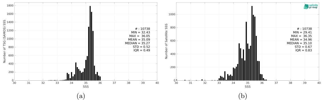
Figure 2: Histograms of SSS from TSG (SAMOS) (a) and Aquarius SSS L2 OR v5 (NASA-GSFC) (b) considering all match-up pairs per bins of 0.1 over the South Pacific Ocean Pi-MEP region and for the full satellite product period.
