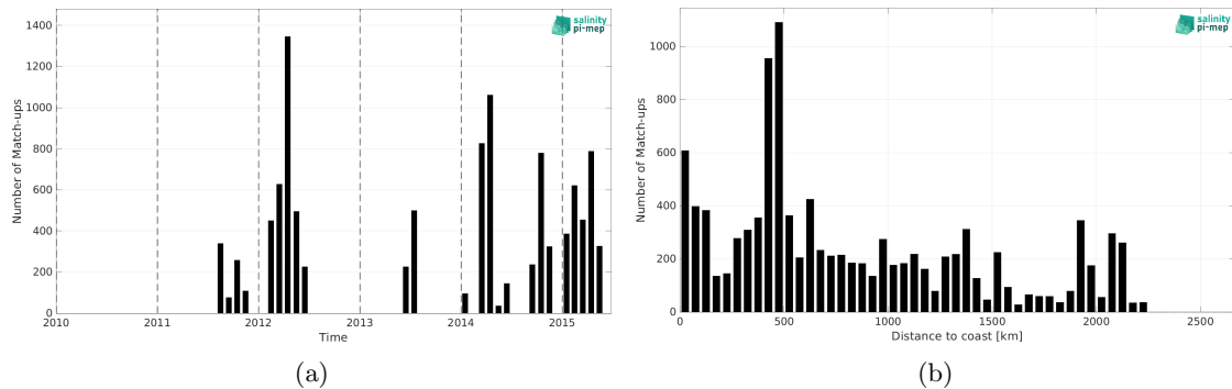
Figure 1: Number of match-ups between TSG (SAMOS) and Aquarius SSS L2 OR v5 (NASA-GSFC) SSS as a function of time (a) and as function of the distance to coast (b) over the South Pacific Ocean Pi-MEP region and for the full satellite product period.
