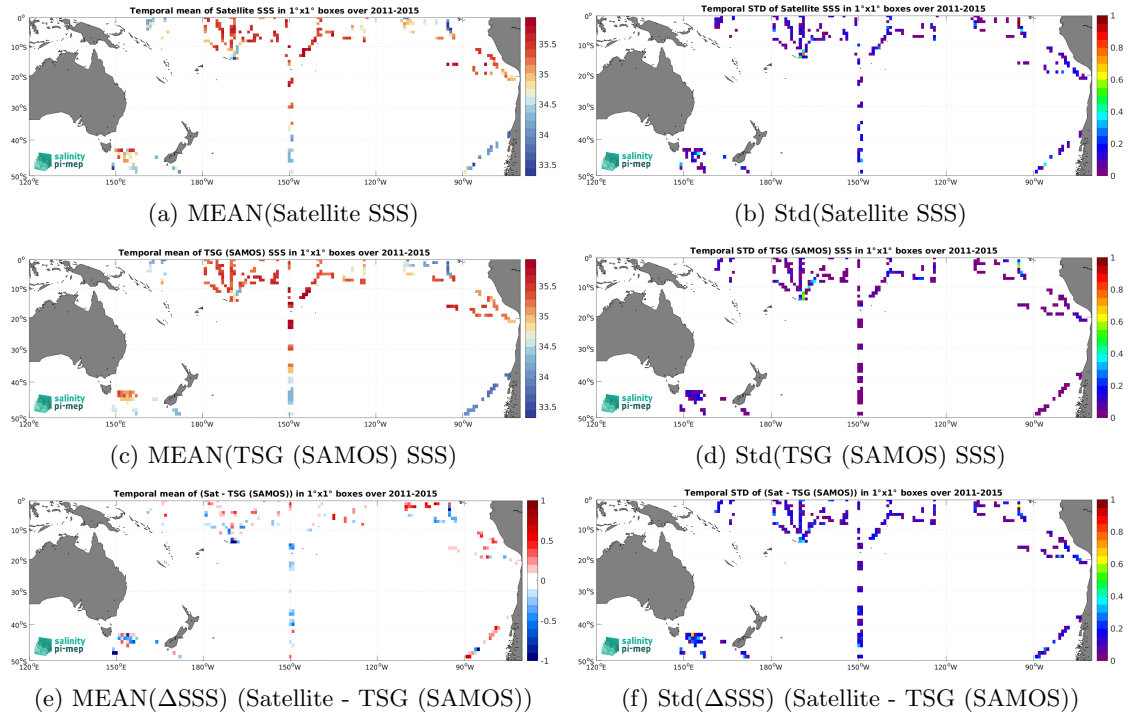
Figure 6: Temporal mean (left) and Std (right) of SSS from Aquarius SSS L2 OR v5 (NASA-GSFC) (top), TSG (SAMOS) (middle), and of \Delta SSS (Satellite - TSG (SAMOS)). Only match-up pairs are used to generate these maps.
