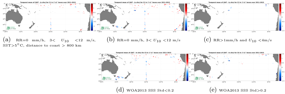
Figure 12: Temporal mean gridded over spatial boxes of size 1^\circ \times 1^\circ of \Delta SSS (Aquarius SSS L2 OR v5 (NASA-GSFC) - TSG (SAMOS)) for 5 different subdatasets corresponding to:RR=0 mm/h, 3 < U_{10} < 12 m/s, SST >5^\circ\text{C} , distance to coast > 800 km (a), RR=0 mm/h, 3 < U_{10} < 12 m/s (b), RR >1 mm/h and U_{10} < 4 m/s (c), WOA2013 SSS Std <0.2 (d), WOA2013 SSS Std >0.2 (e).
