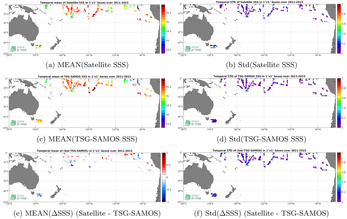
Figure 6: Temporal mean (left) and Std (right) of SSS from Aquarius-L2-OR-V5 (top), TSG-SAMOS (middle), and of \Delta SSS (Satellite - TSG-SAMOS). Only match-up pairs are used to generate these maps.
