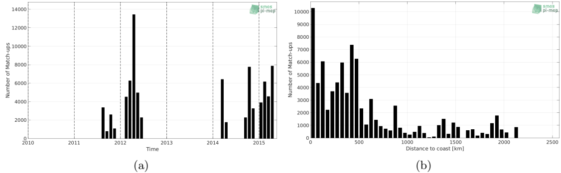
Figure 1: Number of match-ups between TSG-SAMOS and Aquarius-L2-OR-V5 SSS as a function of time (a) and as function of the distance to coast (b) over the South Pacific Ocean Pi-MEP region and for the full satellite product period.
