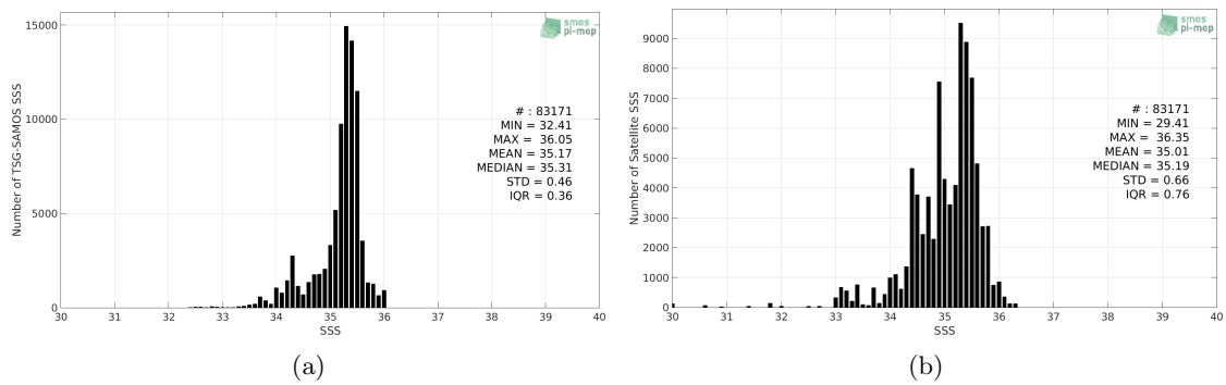
Figure 2: Histograms of SSS from TSG-SAMOS (a) and Aquarius-L2-OR-V5 (b) considering all match-up pairs per bins of 0.1 over the South Pacific Ocean Pi-MEP region and for the full satellite product period.
