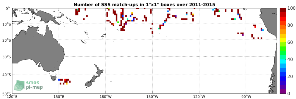
Figure 4: Number of SSS match-ups between TSG-SAMOS SSS and the Aquarius-L2-OR-V5 SSS product for the South Pacific Ocean Pi-MEP region over 1^\circ \times 1^\circ boxes and for the full satellite product period.
