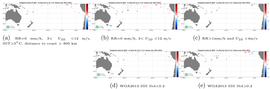
Figure 12: Temporal mean gridded over spatial boxes of size 1^\circ \times 1^\circ of \Delta SSS (Aquarius-L2-OR-V5 - TSG-SAMOS) for 5 different subdatasets corresponding to:RR=0 mm/h, 3 < U_{10} < 12 m/s, SST >5^\circ C, distance to coast > 800 km (a), RR=0 mm/h, 3 < U_{10} < 12 m/s (b), RR >1 mm/h and U_{10} < 4 m/s (c), WOA2013 SSS Std <0.2 (d), WOA2013 SSS Std >0.2 (e).
